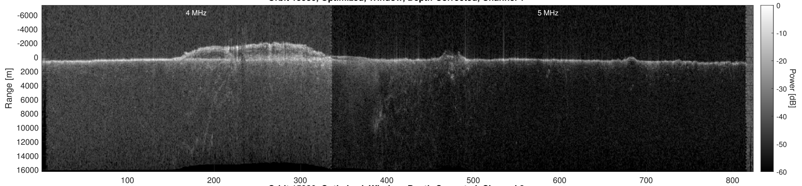
Orbit 15930, Optimized, Window, Depth-Corrected, Channel 2
