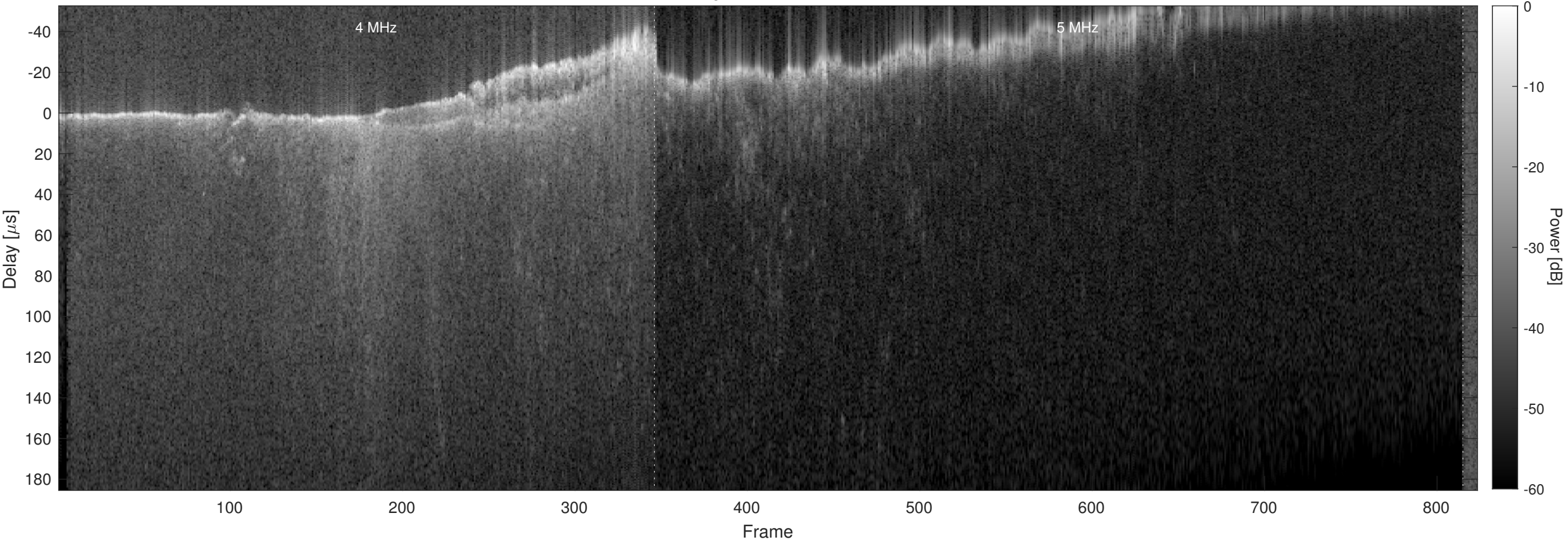
Orbit 15932, Chapman, No Window, Channel 2
