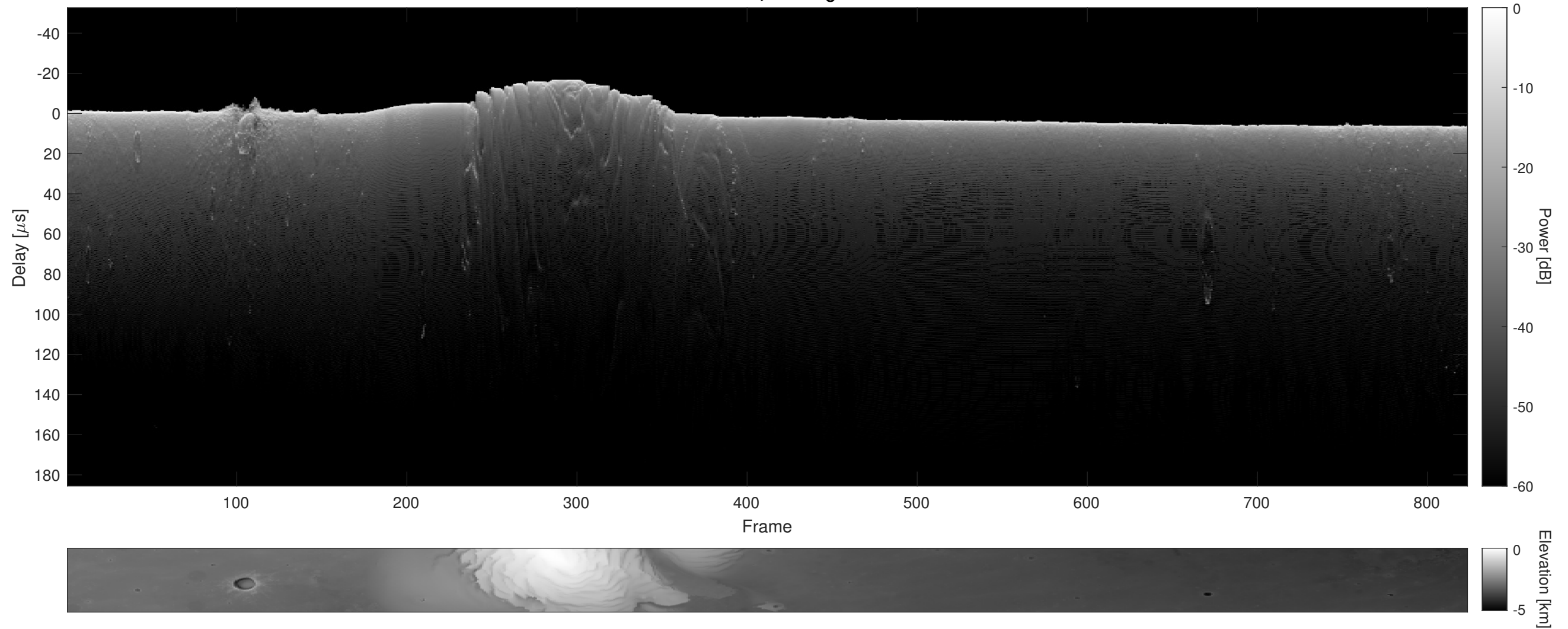
Orbit 15932, Cluttergram
