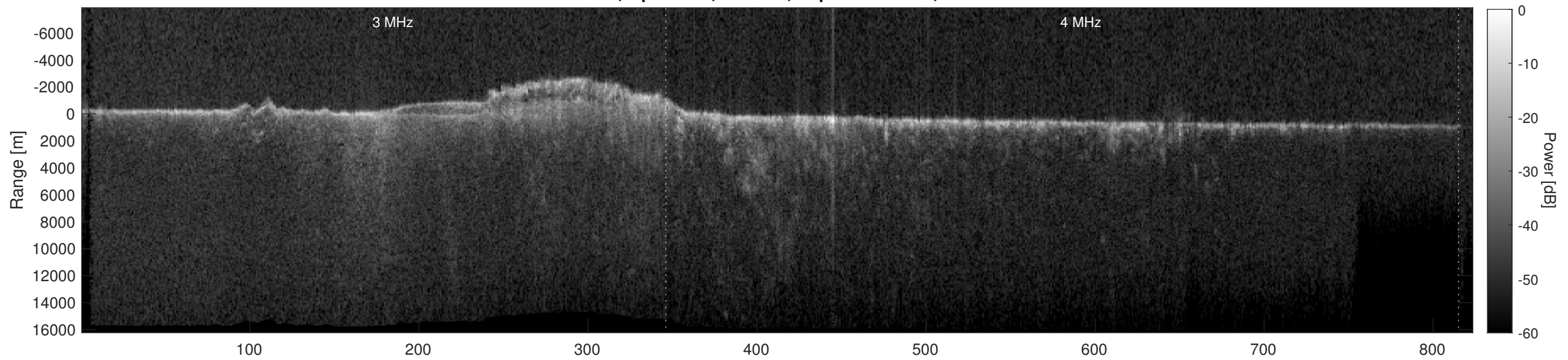
Orbit 15932, Depth-Corrected Cluttergram
