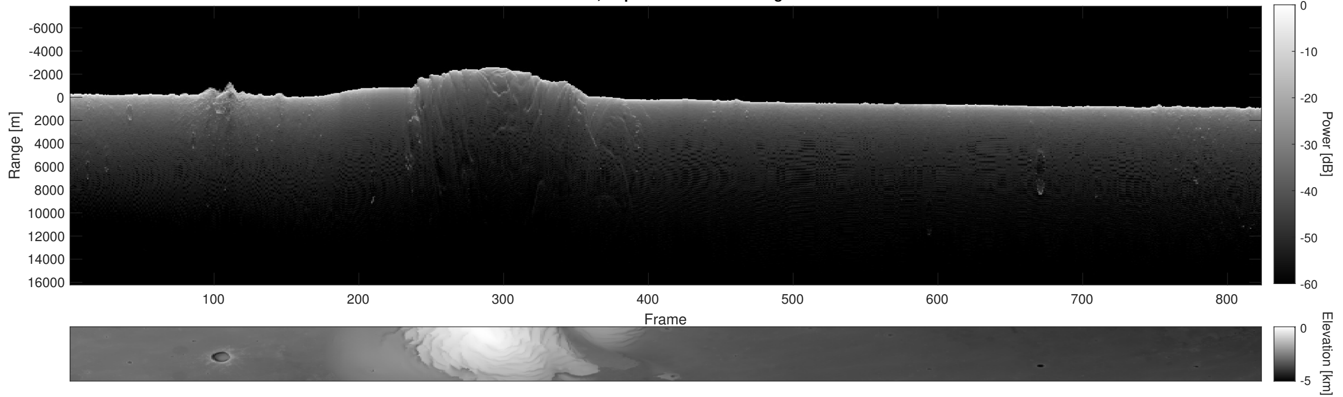
Orbit 15932, Depth-Corrected Cluttergram
