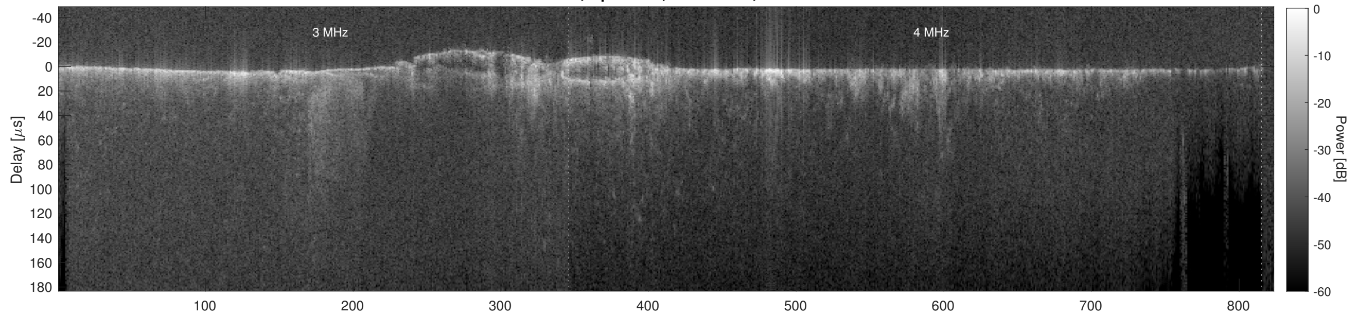
Orbit 15935, Cluttergram
