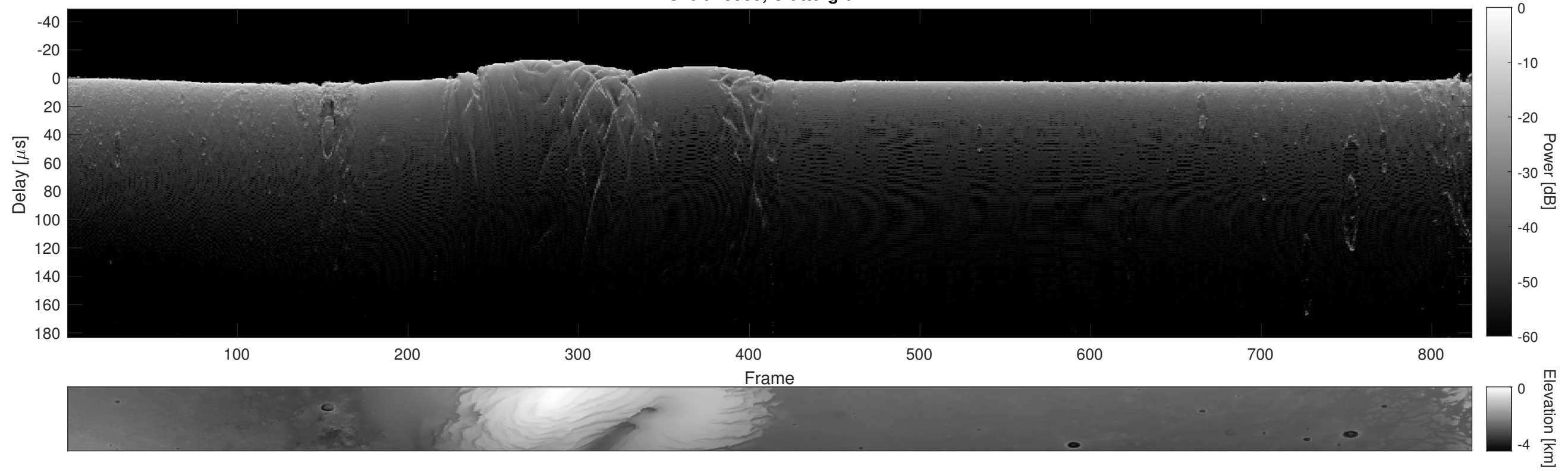
Orbit 15935, Cluttergram
