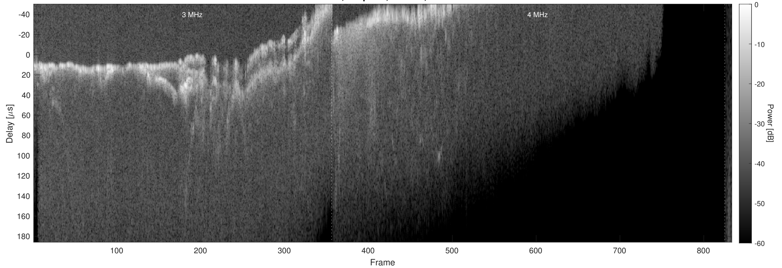
Orbit 15937, Chapman, Window, Channel 2
