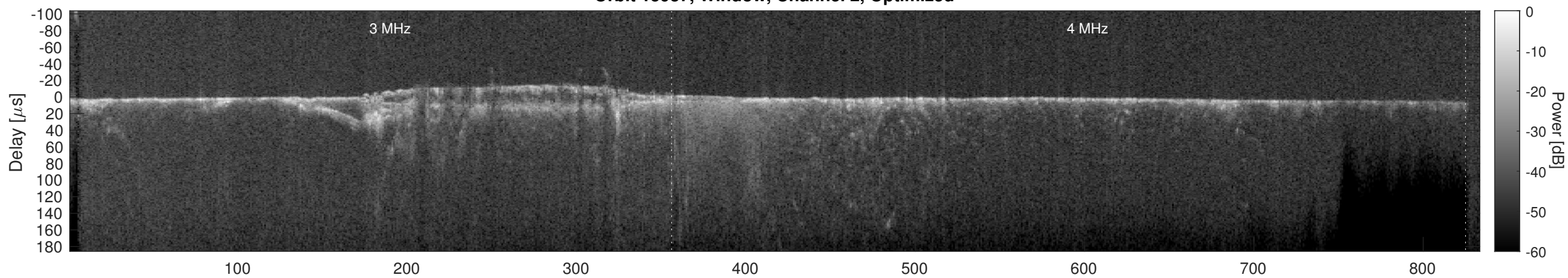
Orbit 15937, Cluttergram
