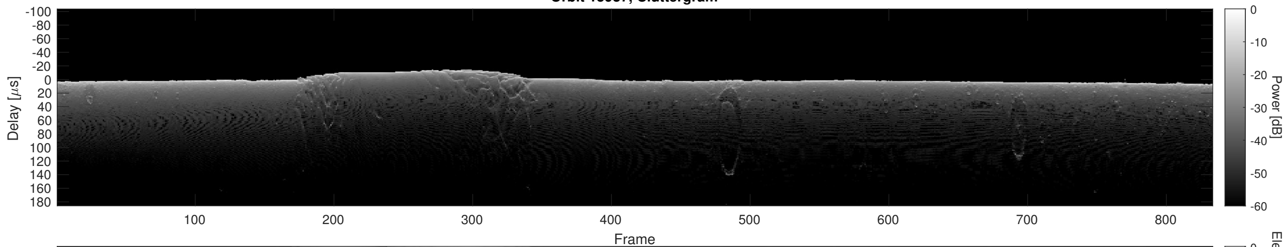
Orbit 15937, Cluttergram
