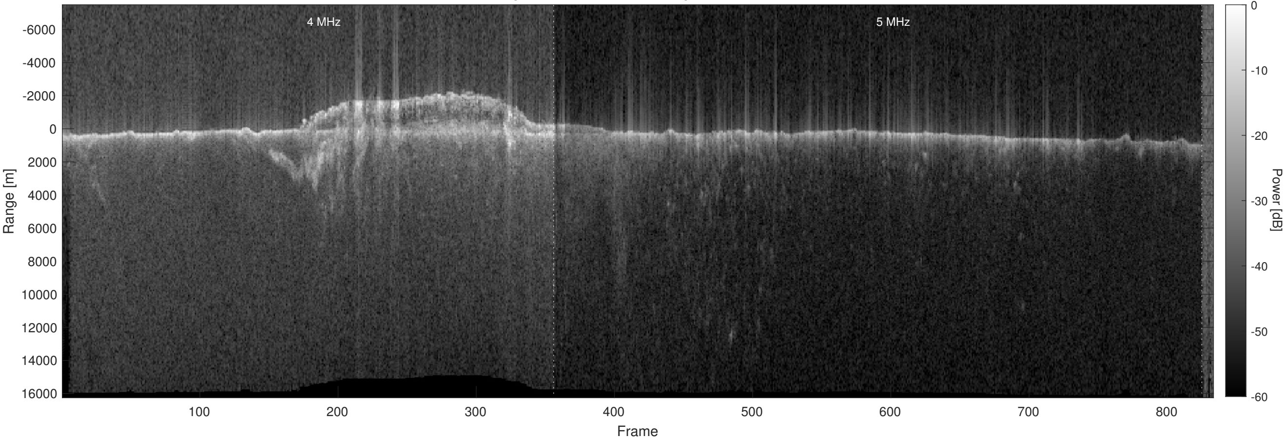
Orbit 15937, Optimized, No Window, Depth-Corrected, Channel 2
