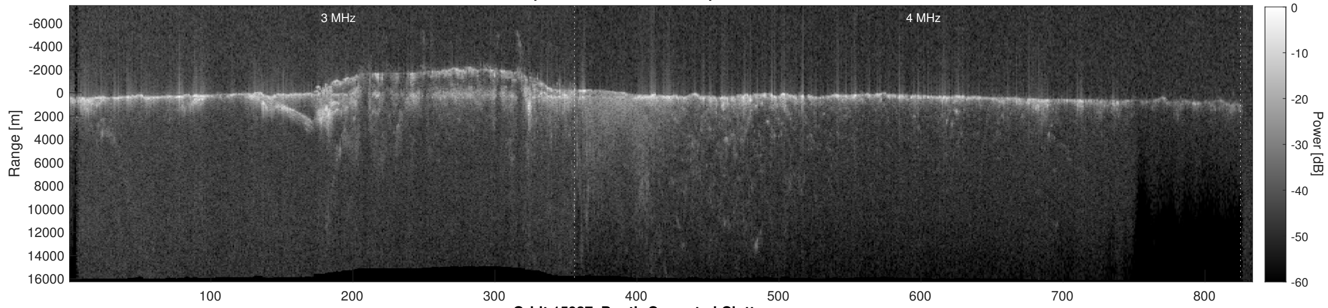
Orbit 15937, Depth-Corrected Cluttergram
