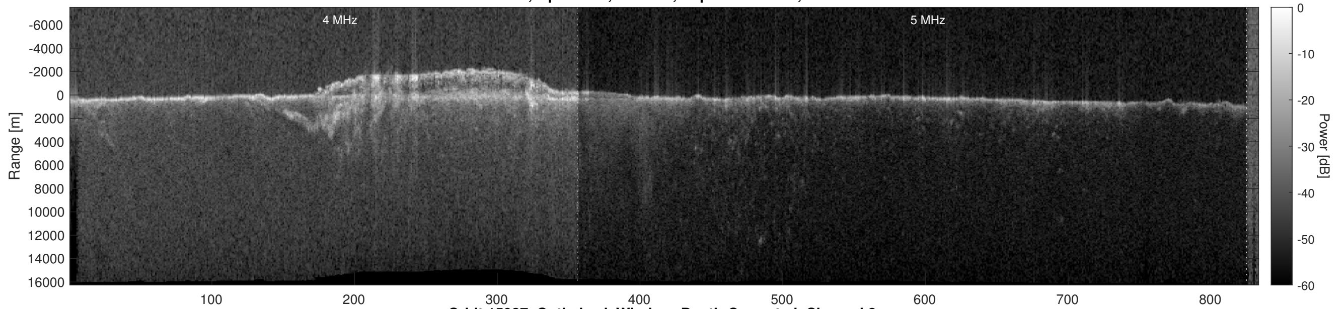
Orbit 15937, Optimized, Window, Depth-Corrected, Channel 2
