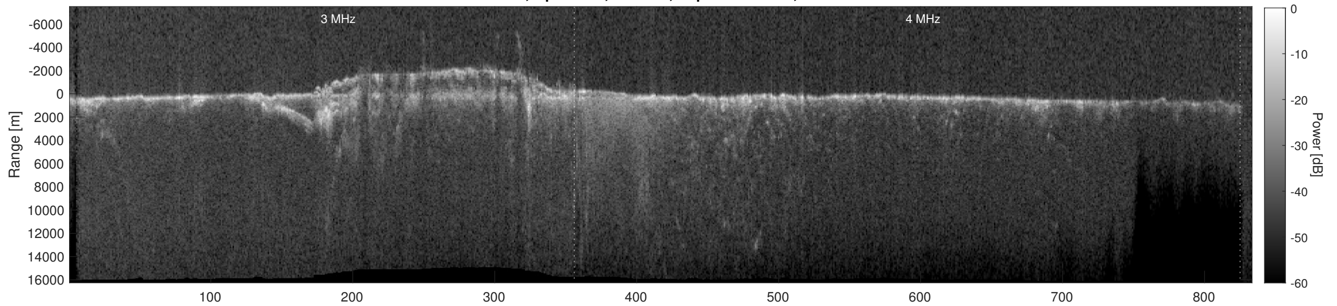
Orbit 15937, Depth-Corrected Cluttergram
