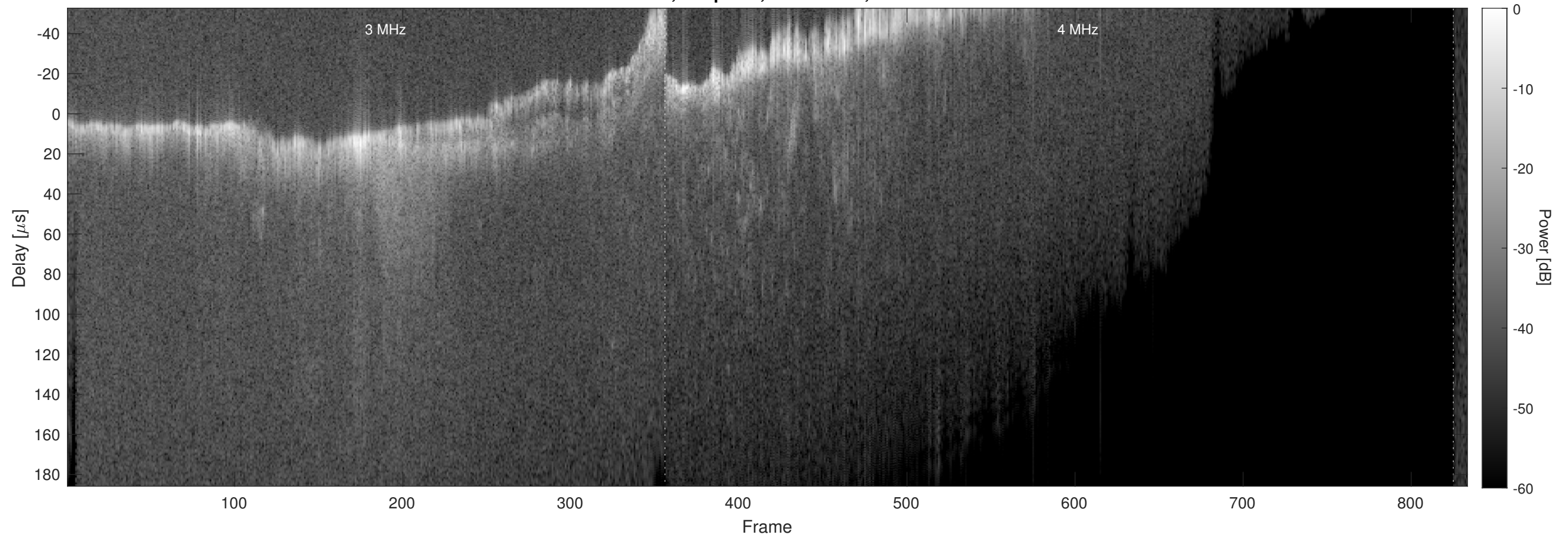
Orbit 15939, Chapman, No Window, Channel 2
