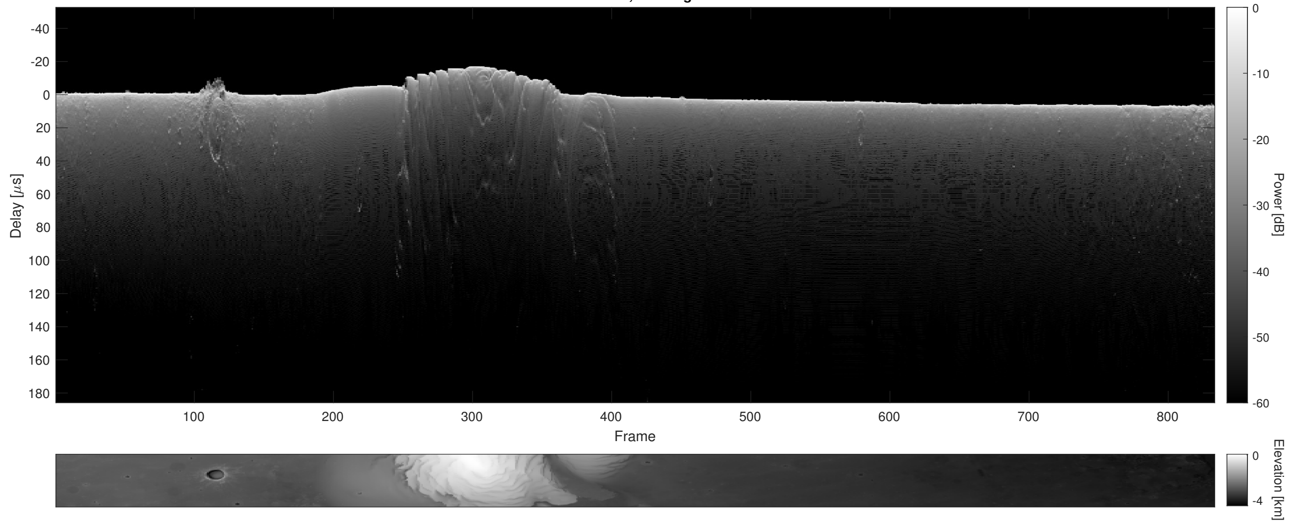
Orbit 15939, Cluttergram
