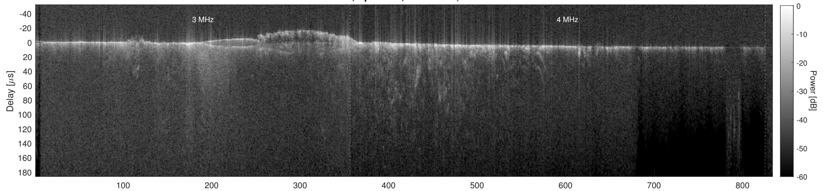
Orbit 15939, Cluttergram
