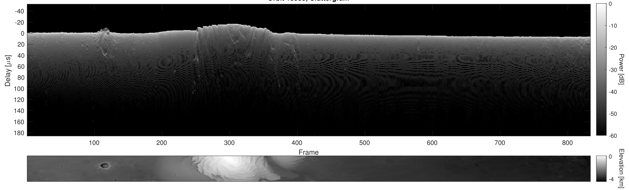
Orbit 15939, Cluttergram
