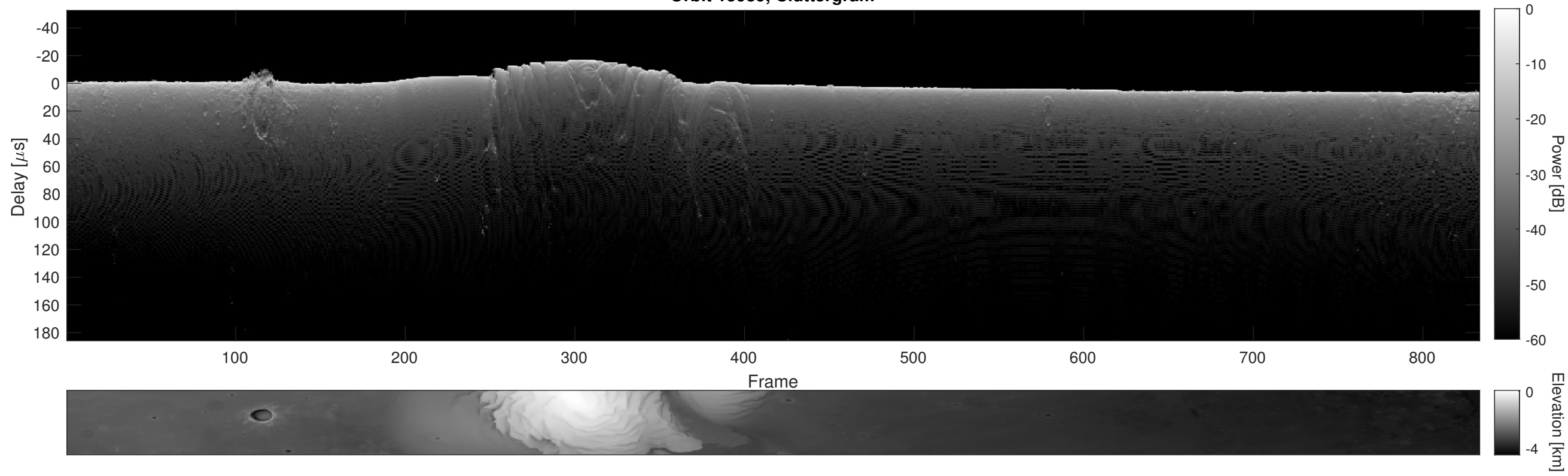
Orbit 15939, Cluttergram
