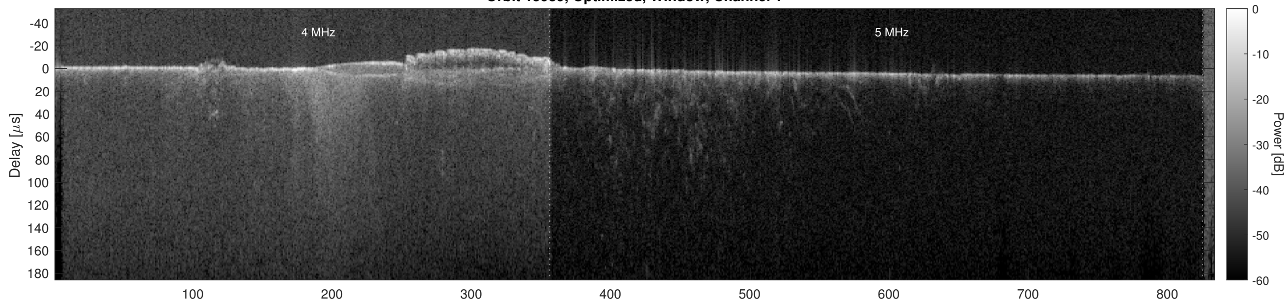
Orbit 15939, Optimized, Window, Channel 2
