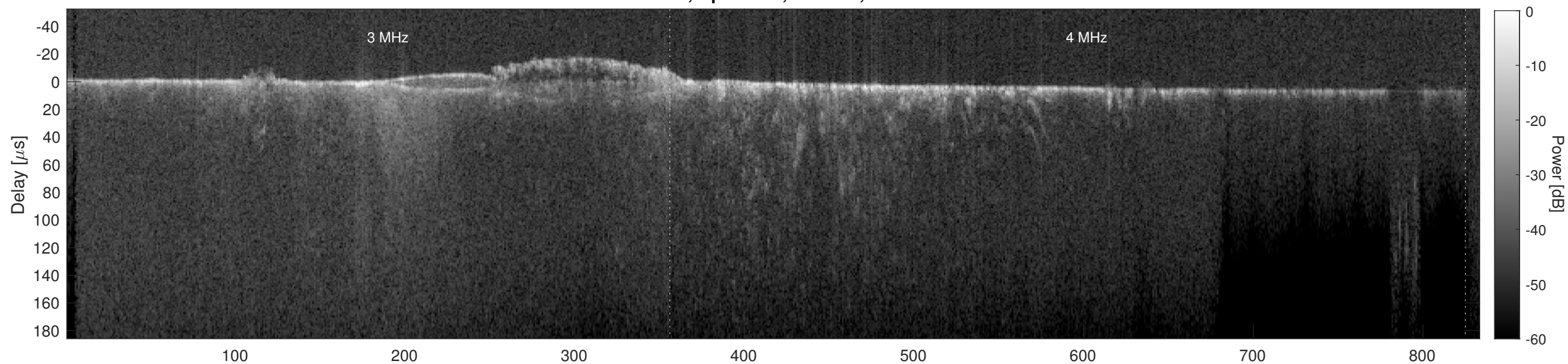
Orbit 15939, Cluttergram
