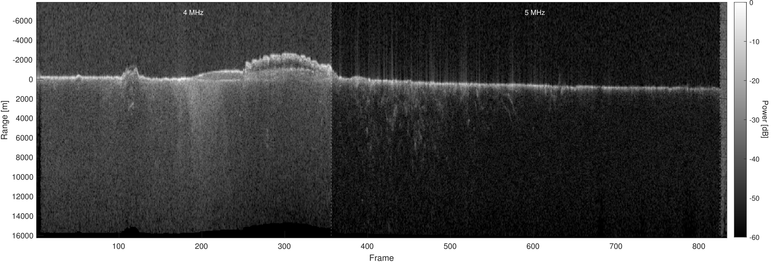
Orbit 15939, Optimized, Window, Depth-Corrected, Channel 2
