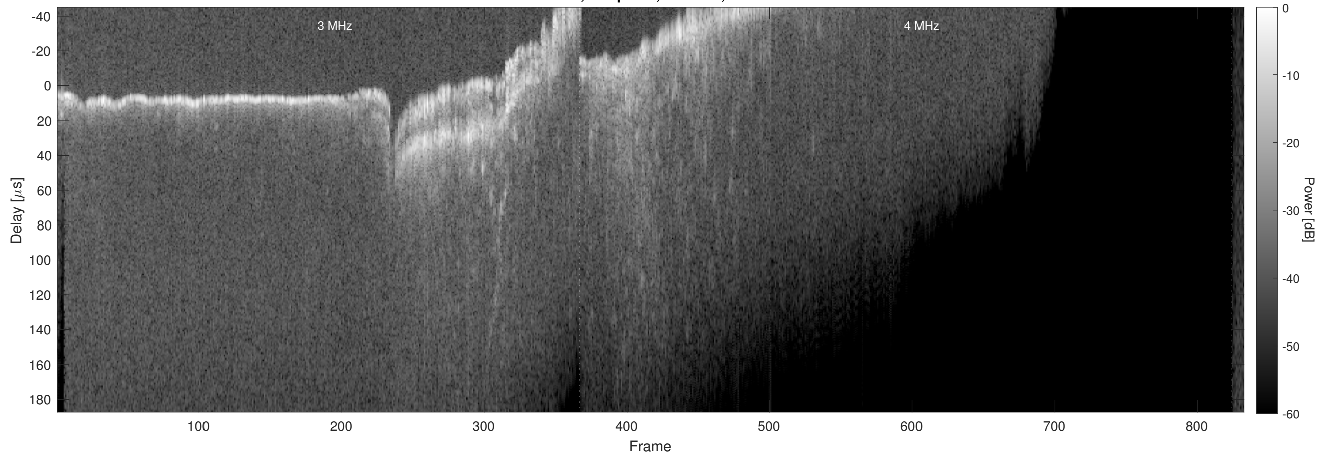
Orbit 15940, Chapman, Window, Channel 2
