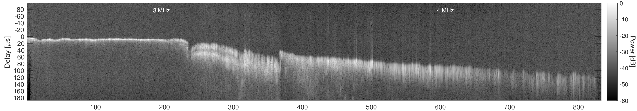
Orbit 15940, Window, Channel 2, Chapman
