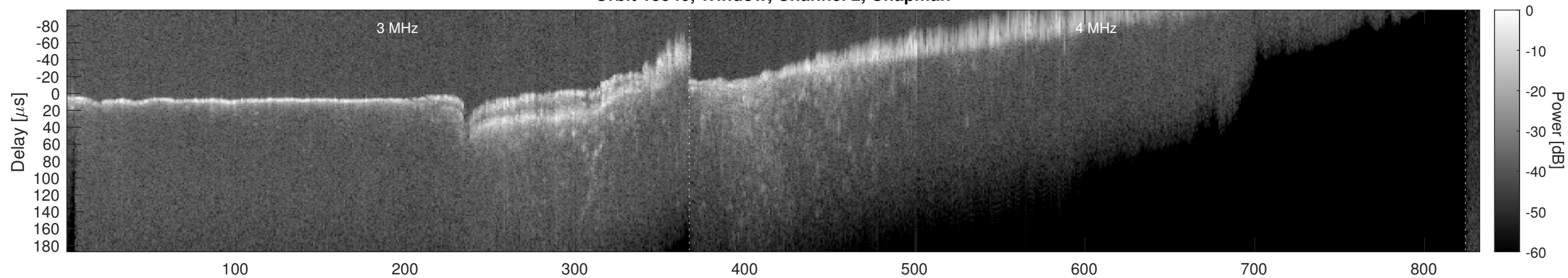
Orbit 15940, Window, Channel 2, Optimized
