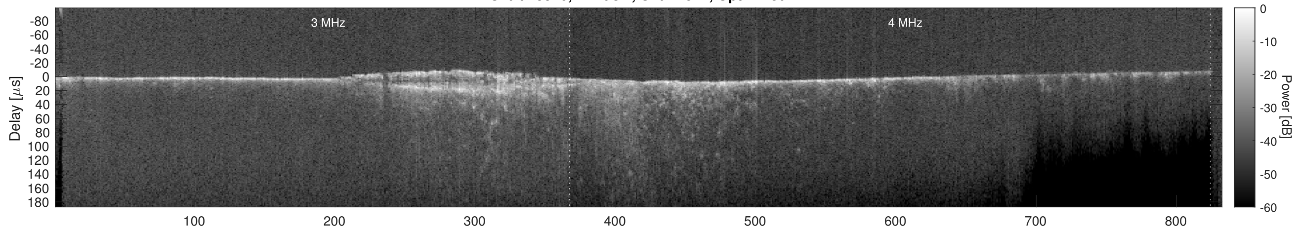
Orbit 15940, Cluttergram
