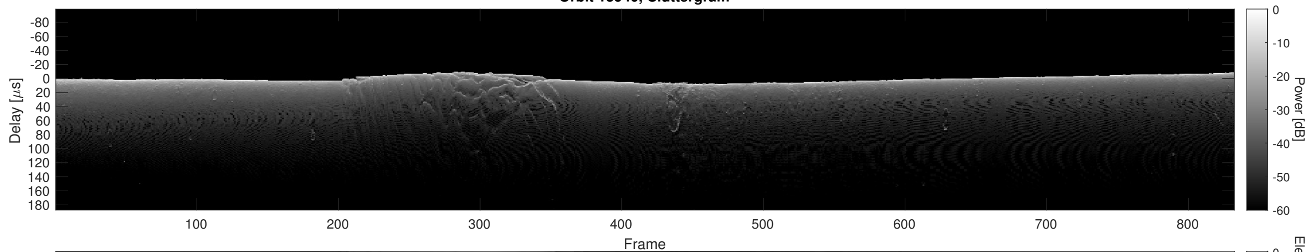
Orbit 15940, Cluttergram
