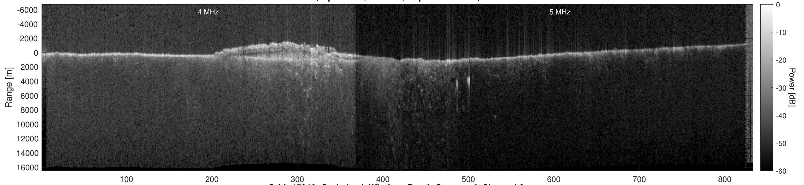
Orbit 15940, Optimized, Window, Depth-Corrected, Channel 2
