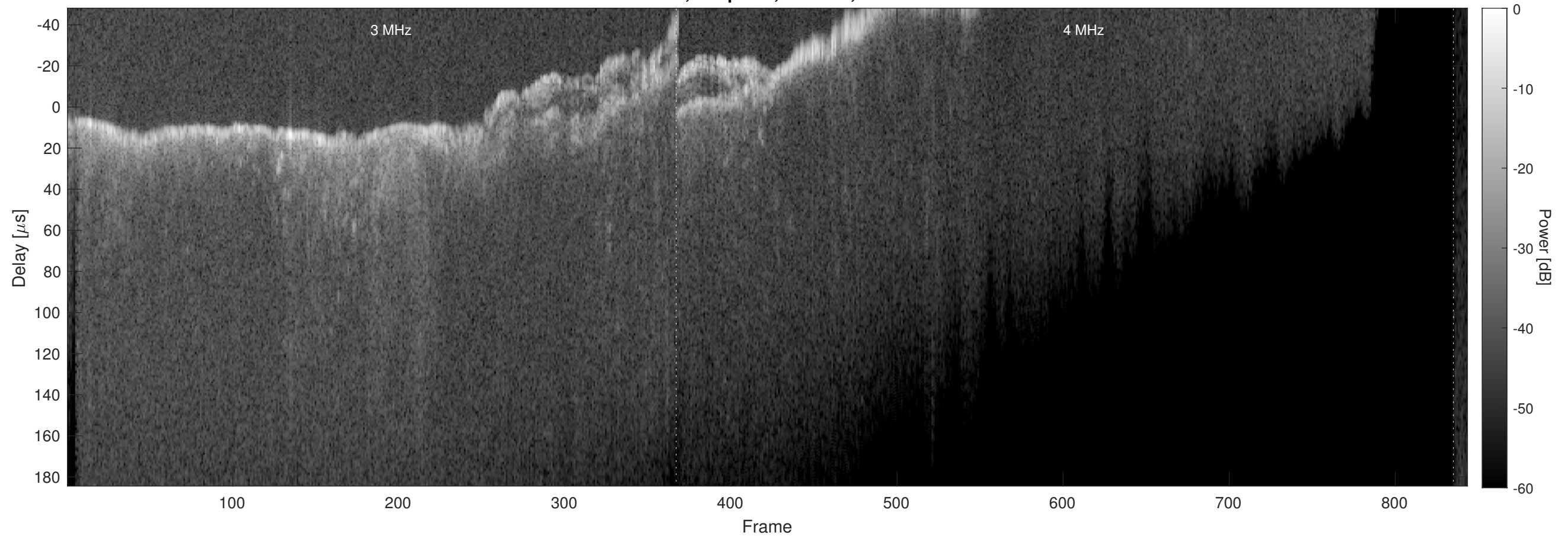
Orbit 15942, Chapman, Window, Channel 2
