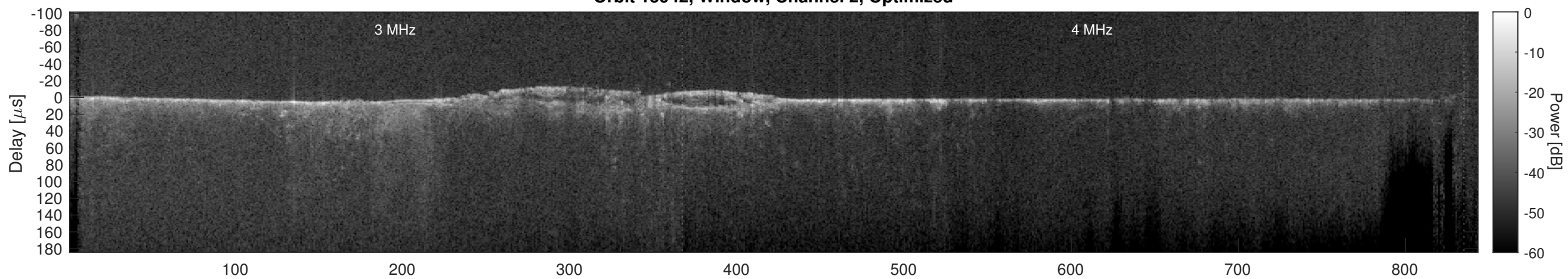
Orbit 15942, Cluttergram
