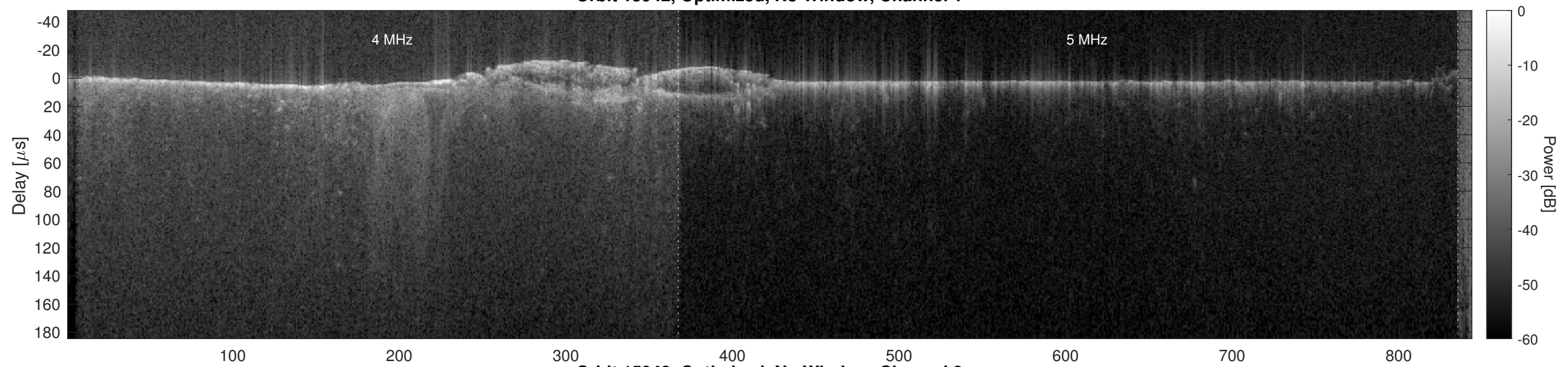
Orbit 15942, Optimized, No Window, Channel 2
