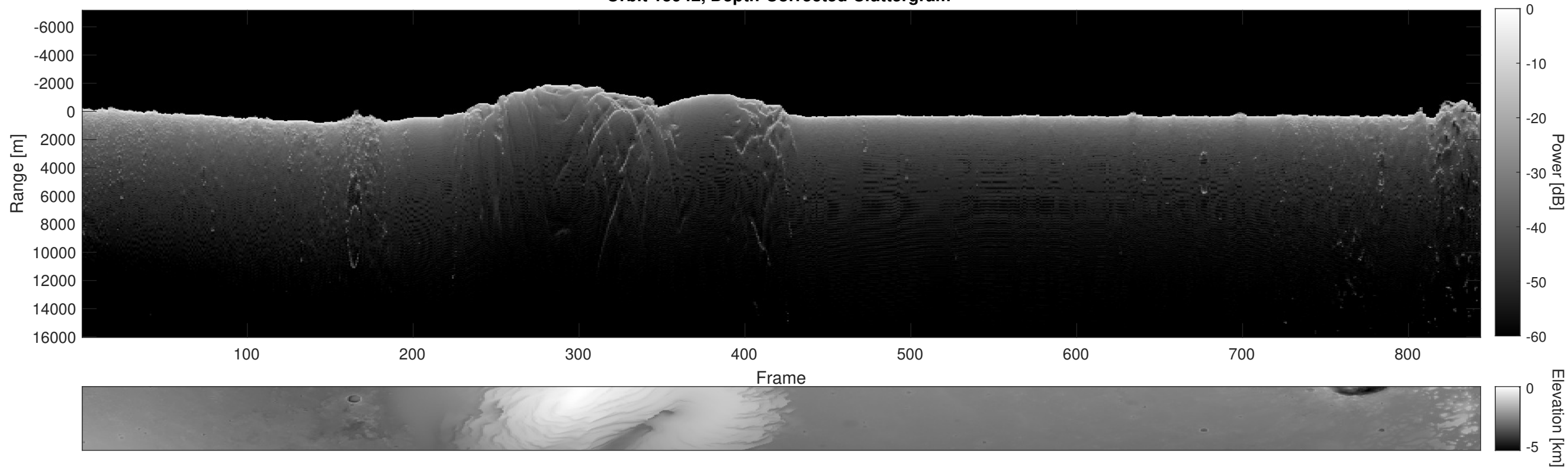
Orbit 15942, Depth-Corrected Cluttergram
