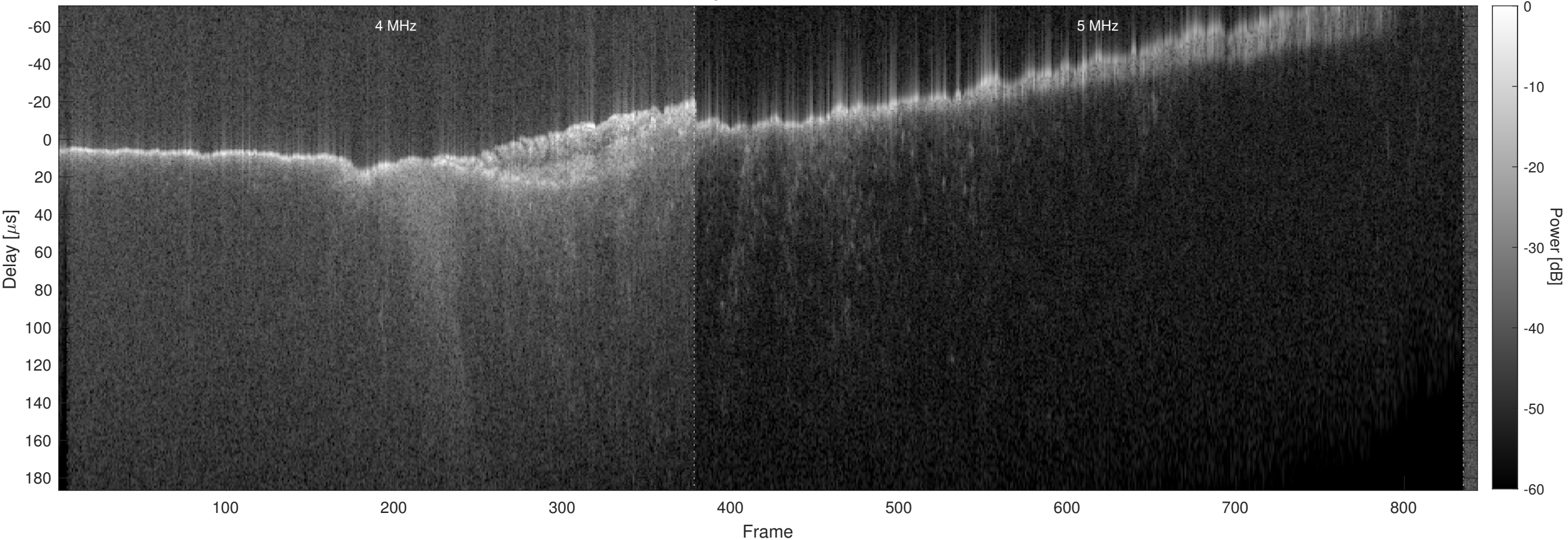
Orbit 15943, Chapman, No Window, Channel 2
