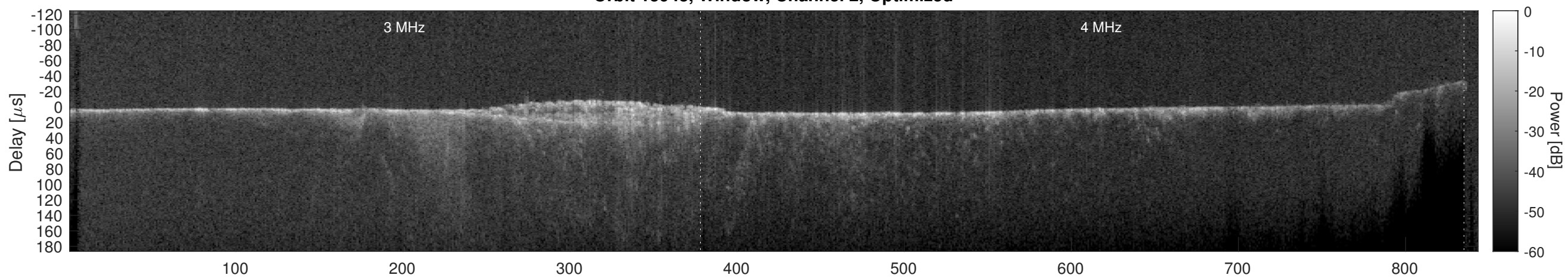
Orbit 15943, Cluttergram
