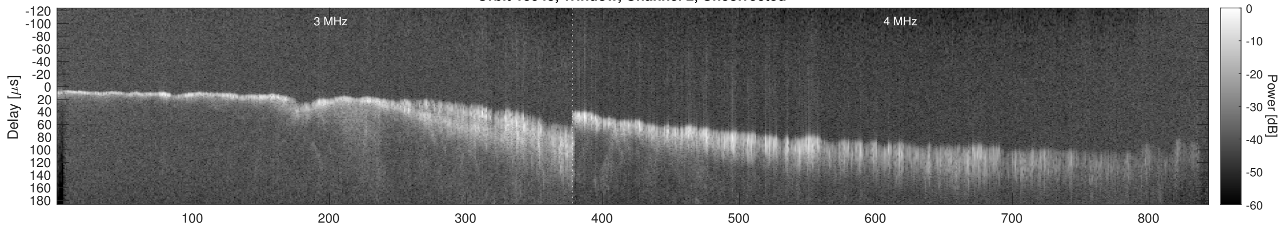
Orbit 15943, Window, Channel 2, Chapman
