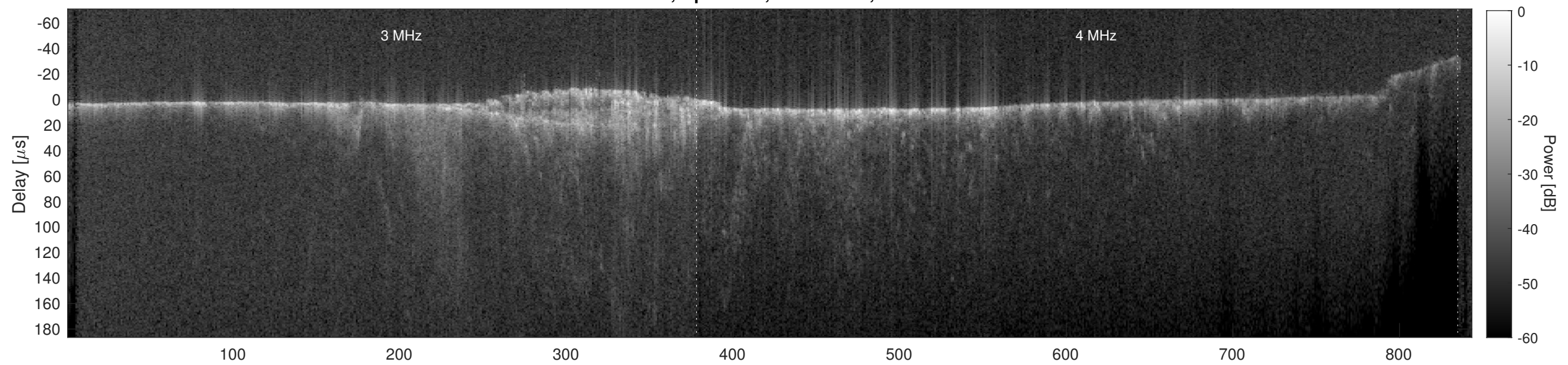
Orbit 15943, Cluttergram
