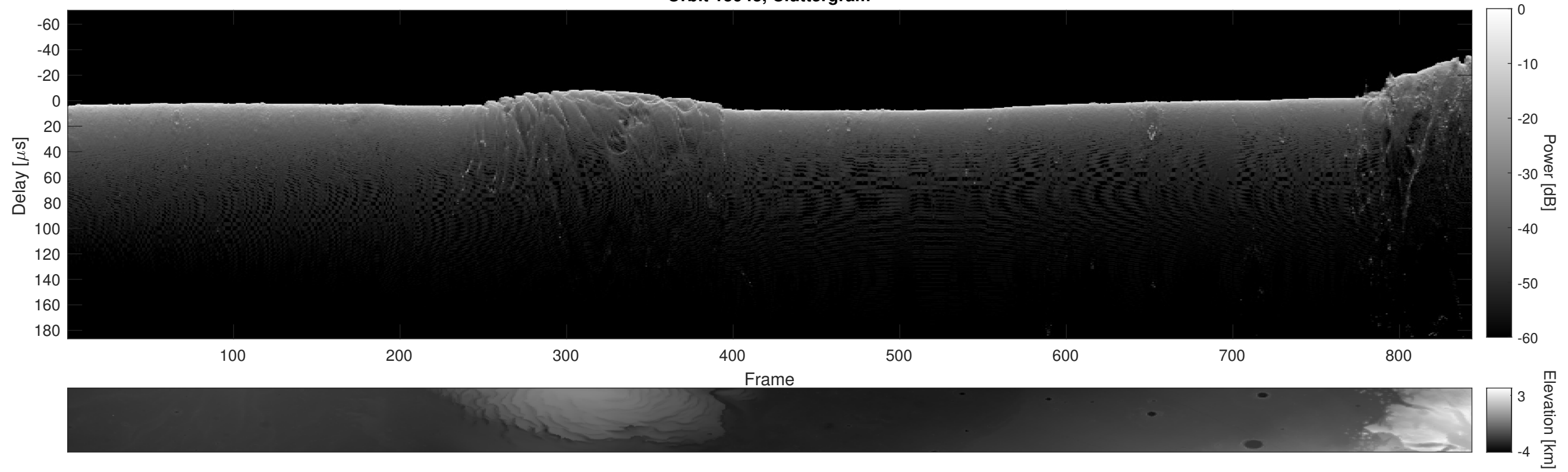
Orbit 15943, Cluttergram
