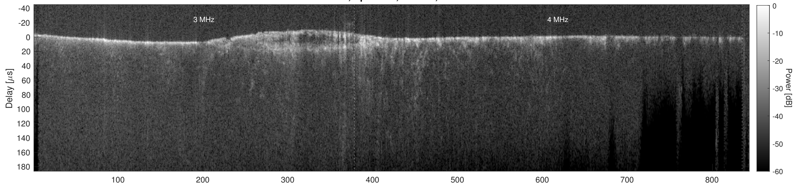
Orbit 15945, Cluttergram
