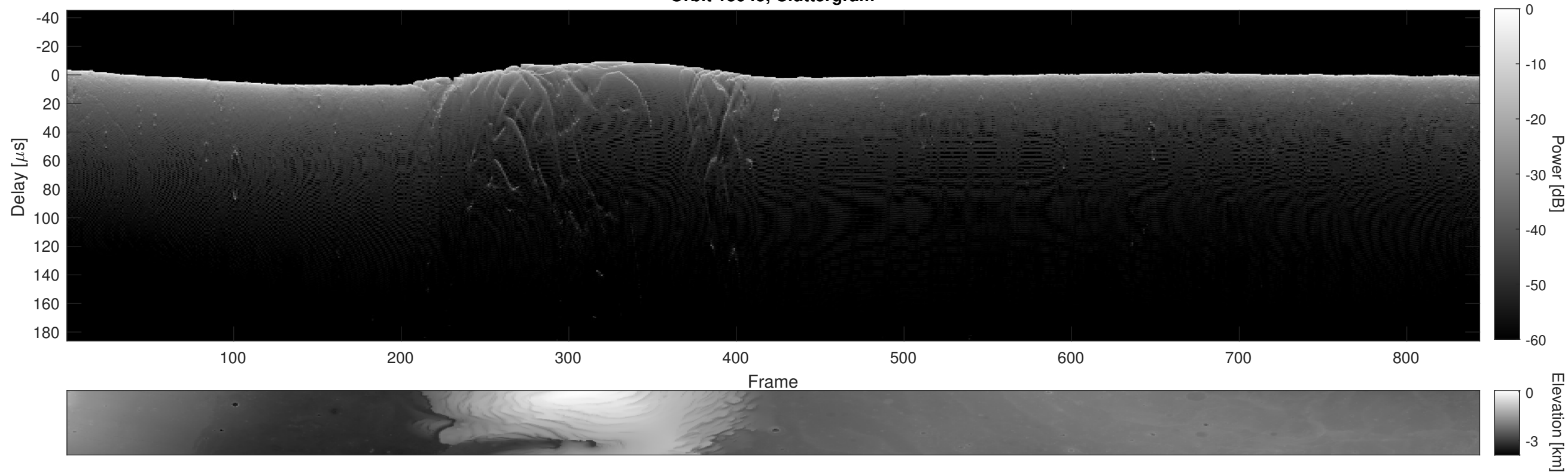
Orbit 15945, Cluttergram
