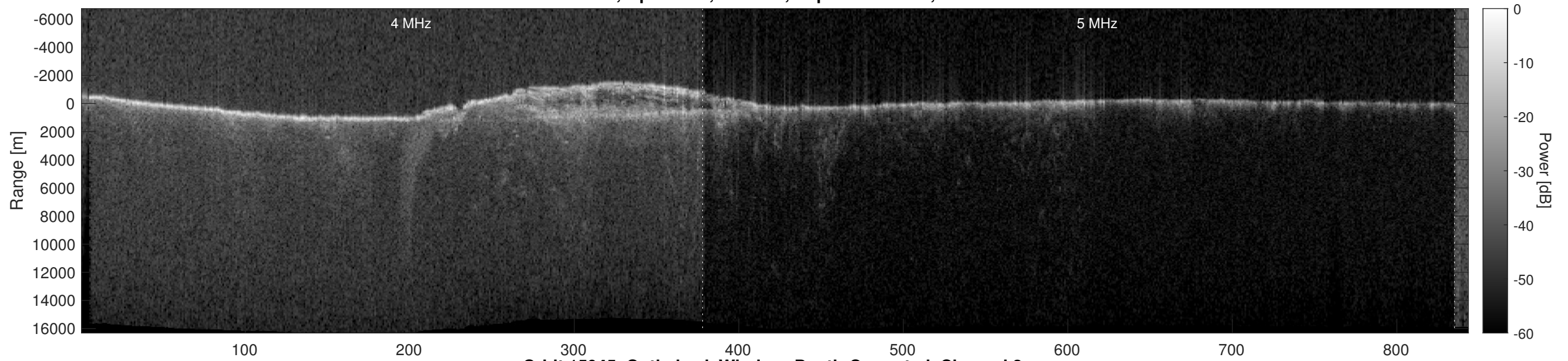
Orbit 15945, Optimized, Window, Depth-Corrected, Channel 2
