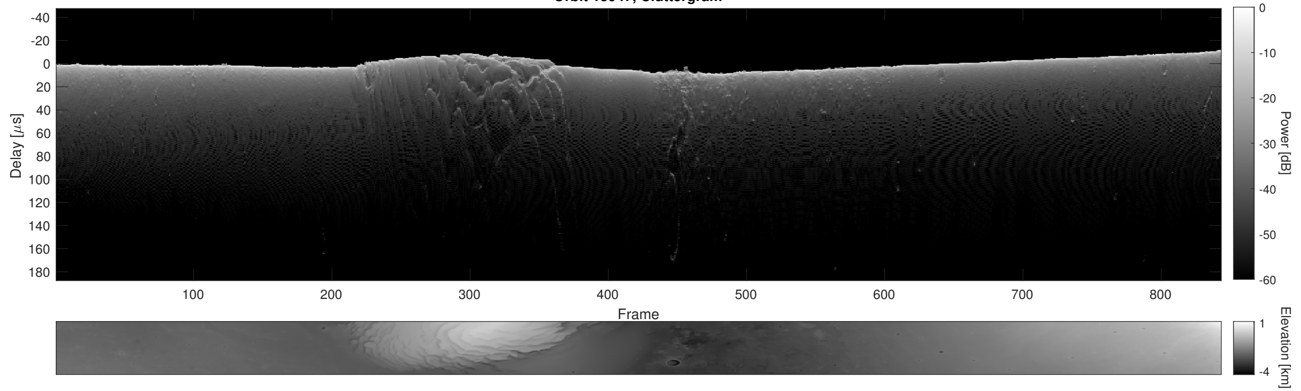
Orbit 15947, Cluttergram
