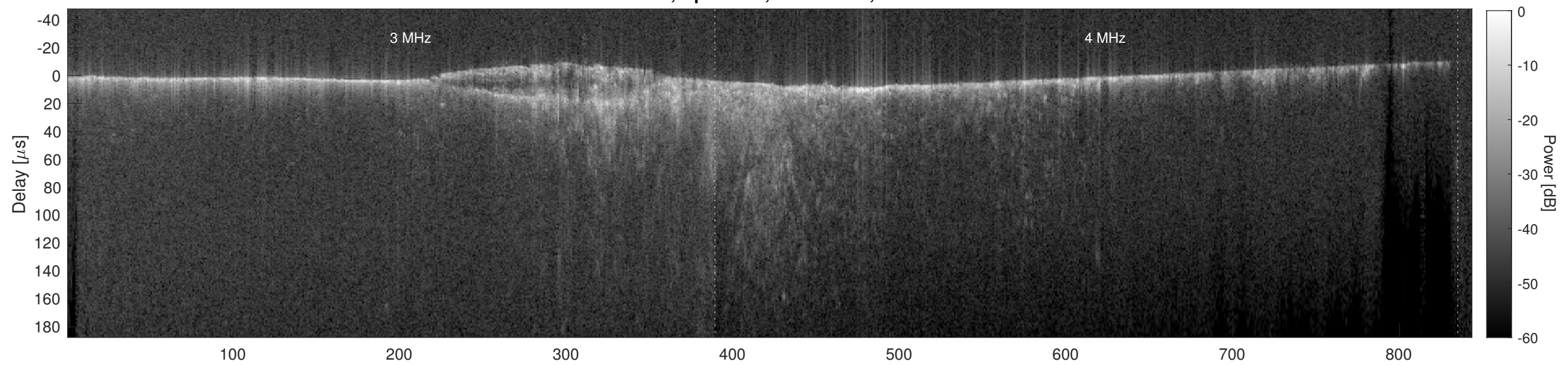
Orbit 15947, Cluttergram
