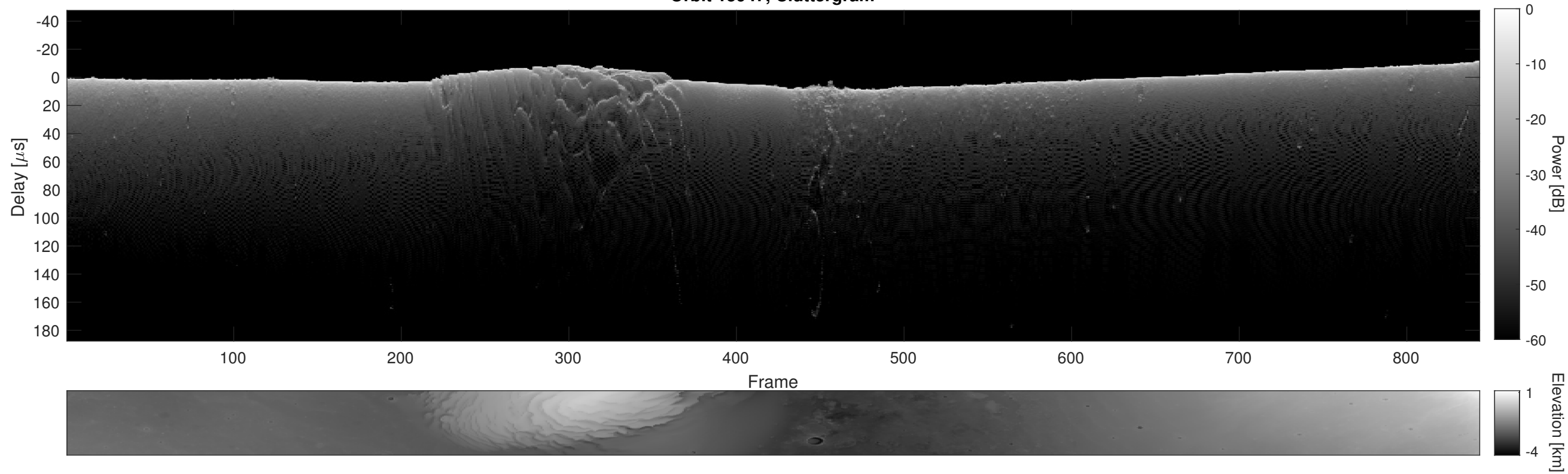
Orbit 15947, Cluttergram
