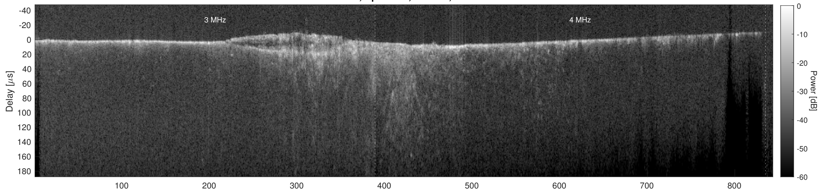
Orbit 15947, Cluttergram
