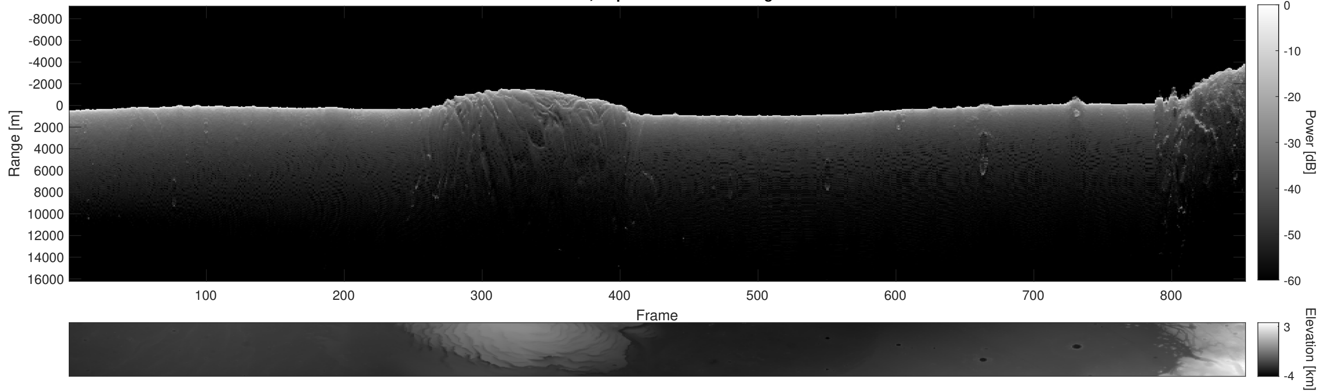
Orbit 15950, Depth-Corrected Cluttergram
