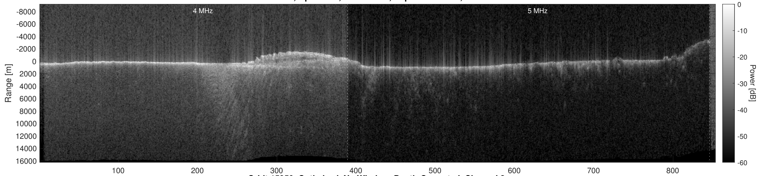
Orbit 15950, Optimized, No Window, Depth-Corrected, Channel 2
