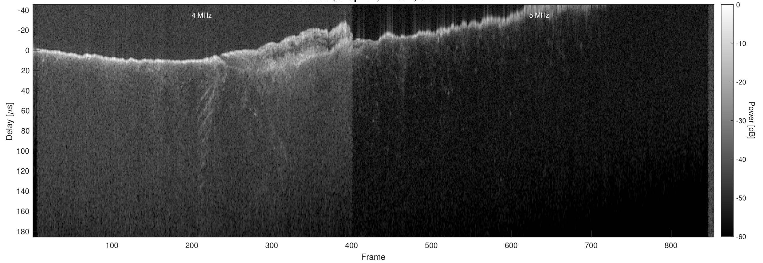
Orbit 15952, Chapman, Window, Channel 2
