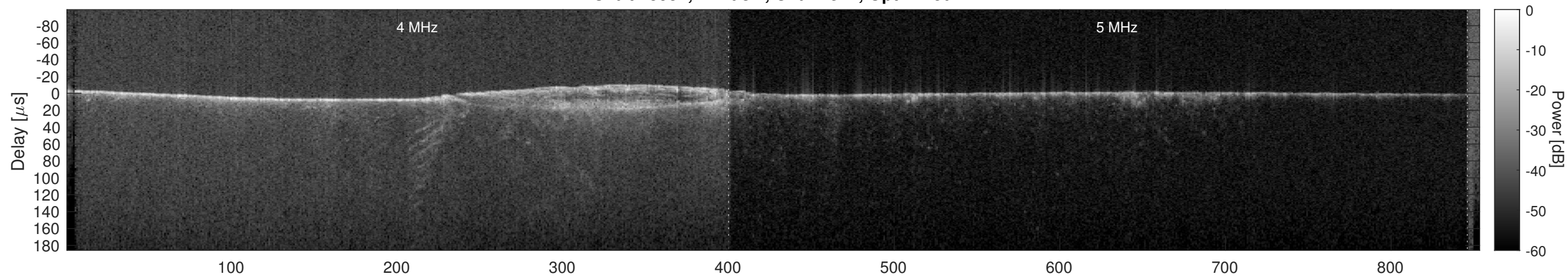
Orbit 15952, Cluttergram
