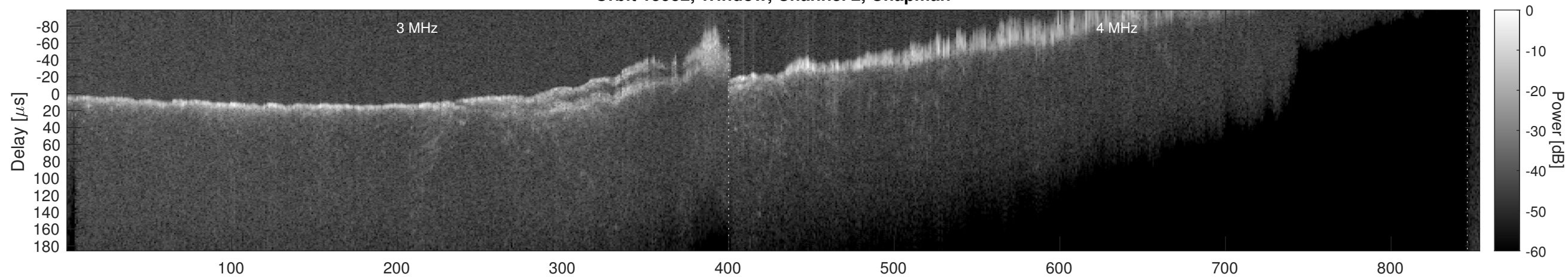
Orbit 15952, Window, Channel 2, Optimized
