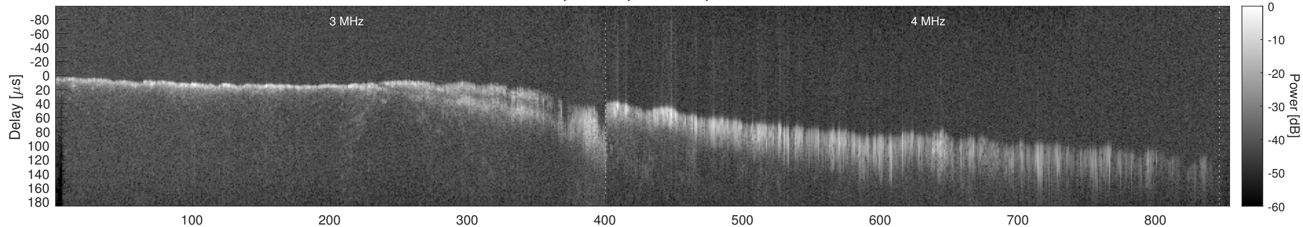
Orbit 15952, Window, Channel 2, Chapman
