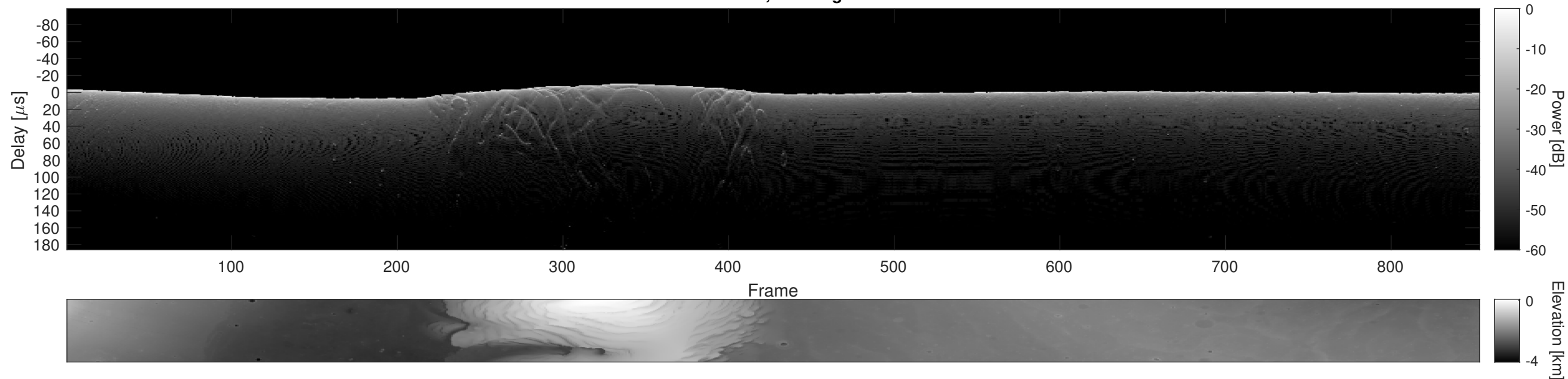
Orbit 15952, Cluttergram
