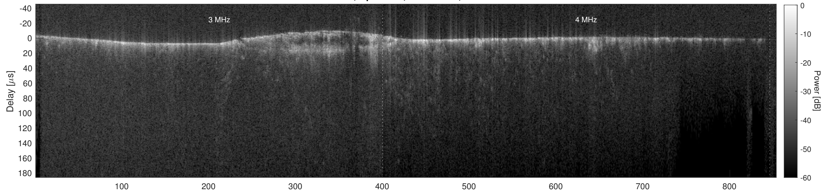
Orbit 15952, Cluttergram
