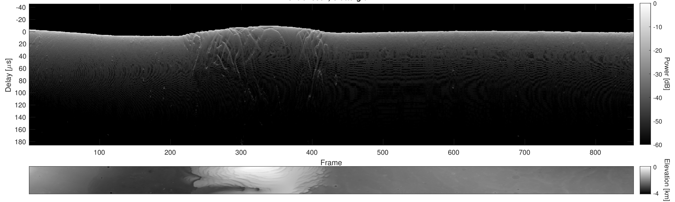
Orbit 15952, Cluttergram
