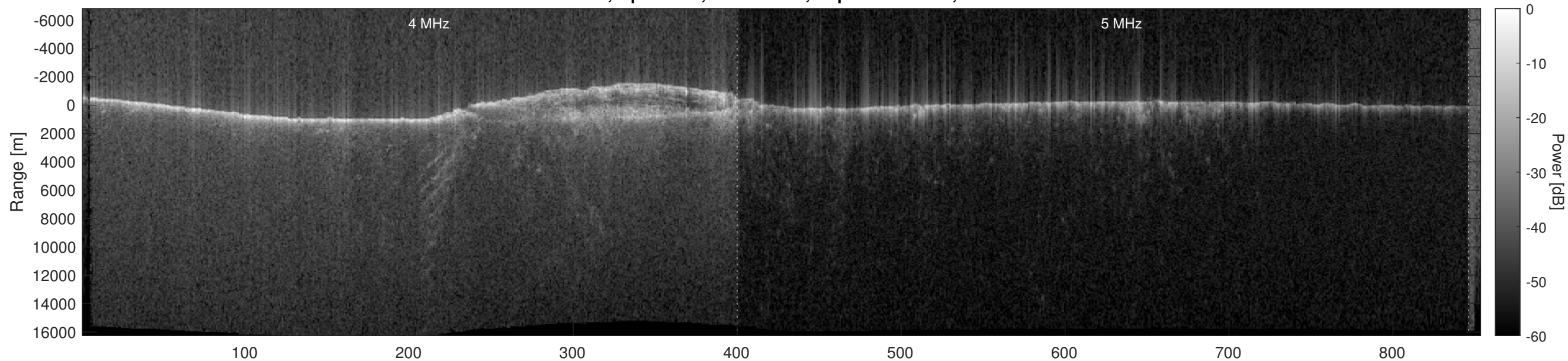
Orbit 15952, Optimized, No Window, Depth-Corrected, Channel 2
