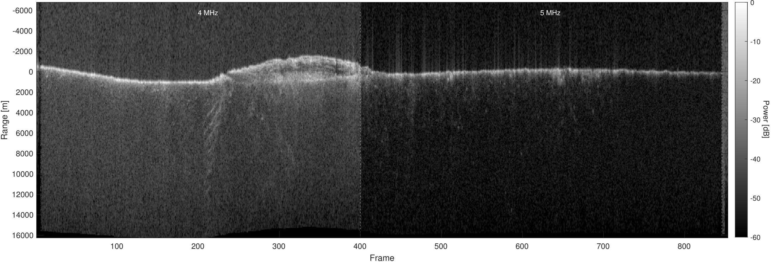
Orbit 15952, Optimized, Window, Depth-Corrected, Channel 2
