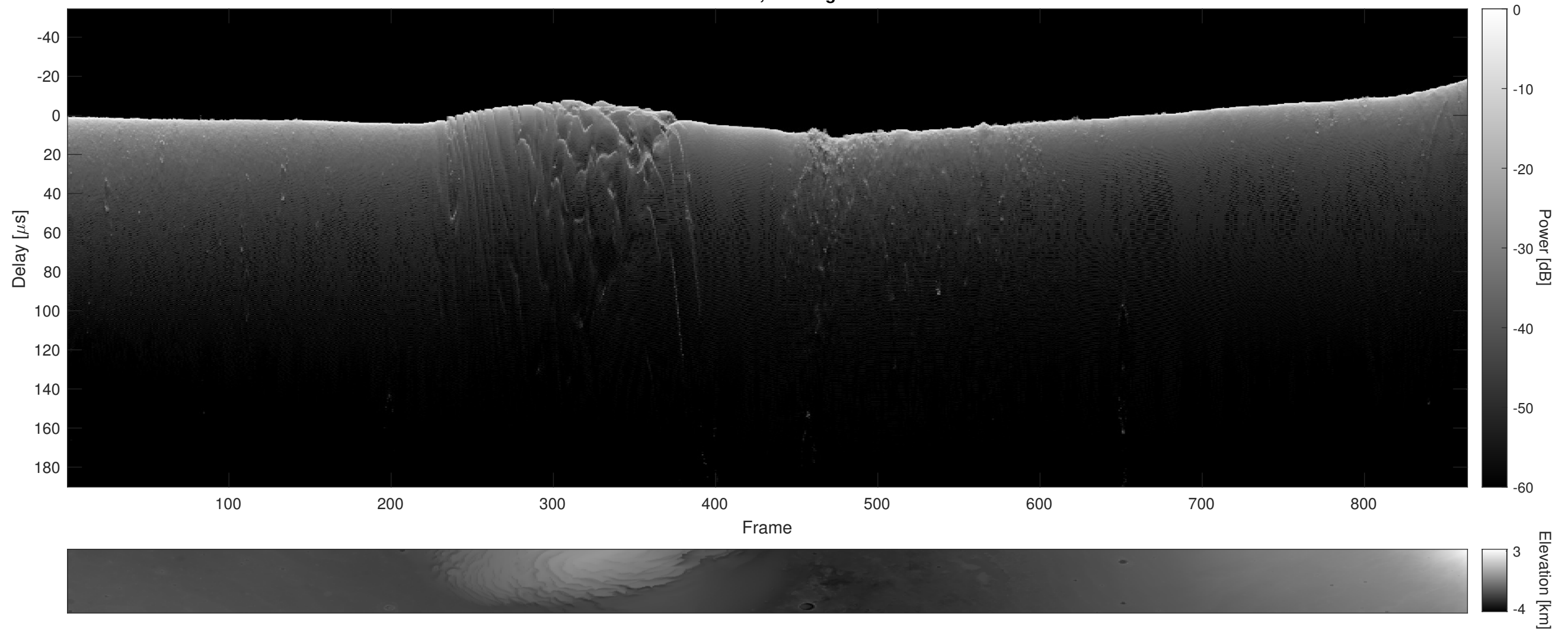
Orbit 15954, Cluttergram
