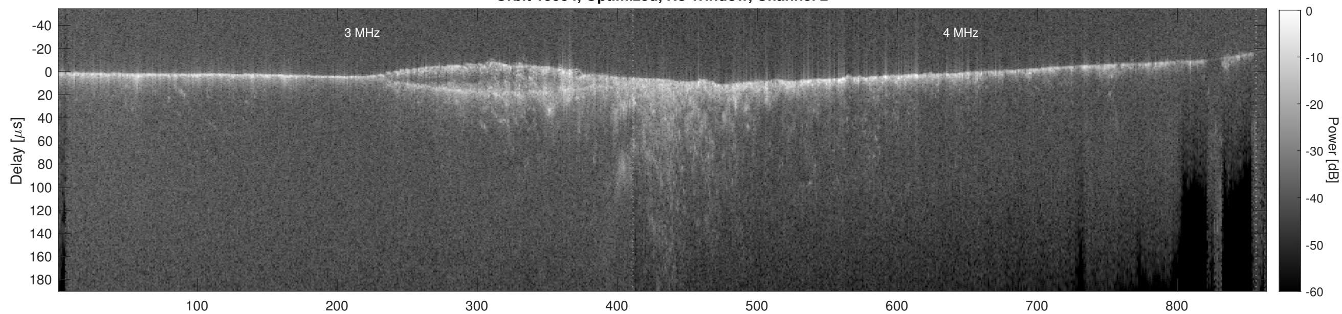
Orbit 15954, Cluttergram
