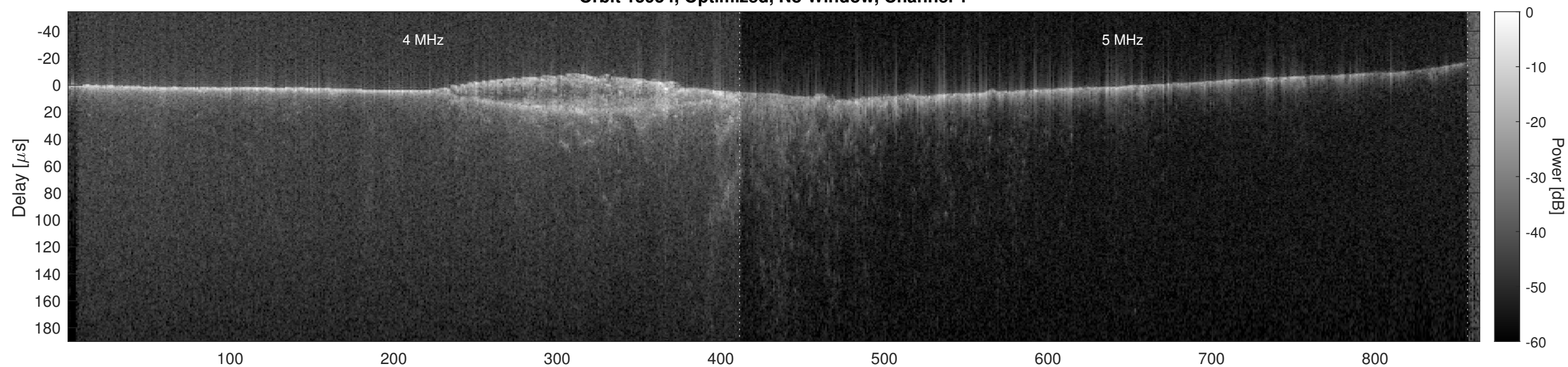
Orbit 15954, Optimized, No Window, Channel 2
