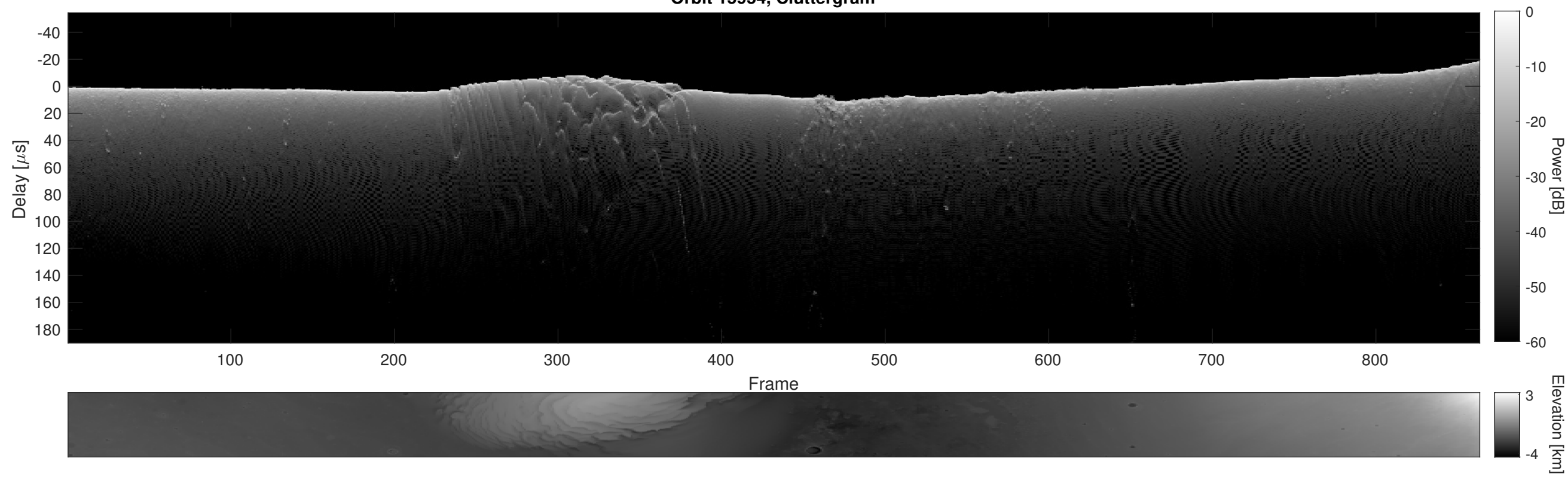
Orbit 15954, Cluttergram
