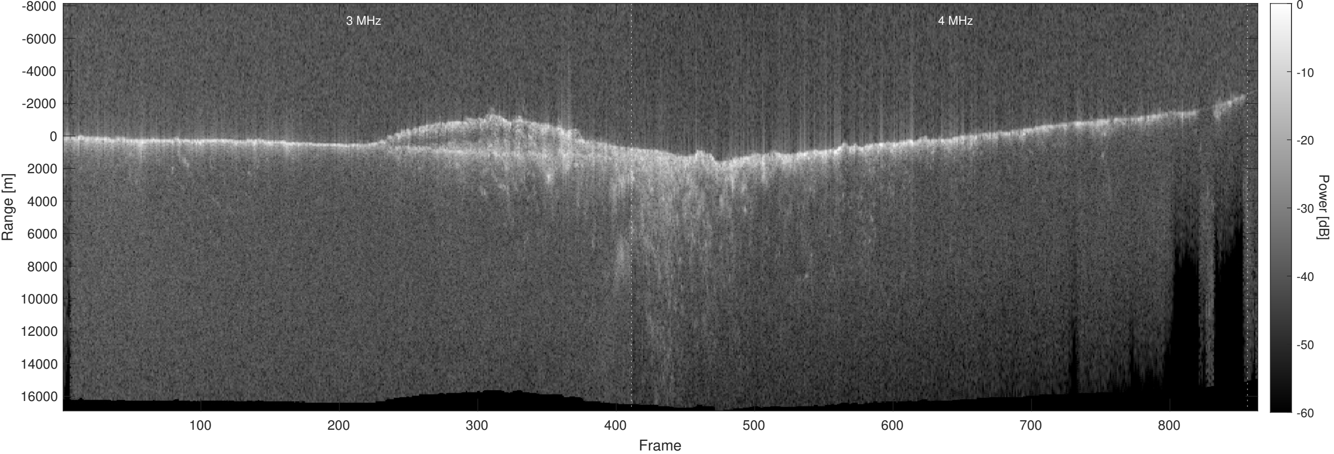
Orbit 15954, Optimized, No Window, Depth-Corrected, Channel 2
