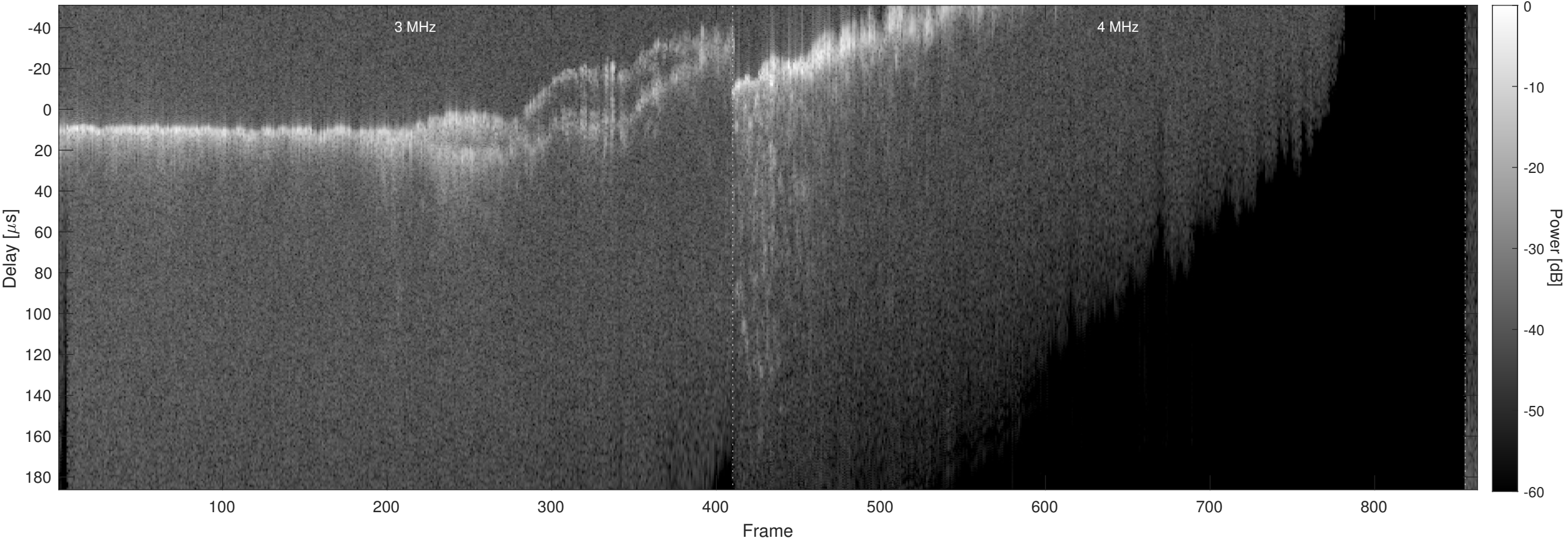
Orbit 15955, Chapman, No Window, Channel 2
