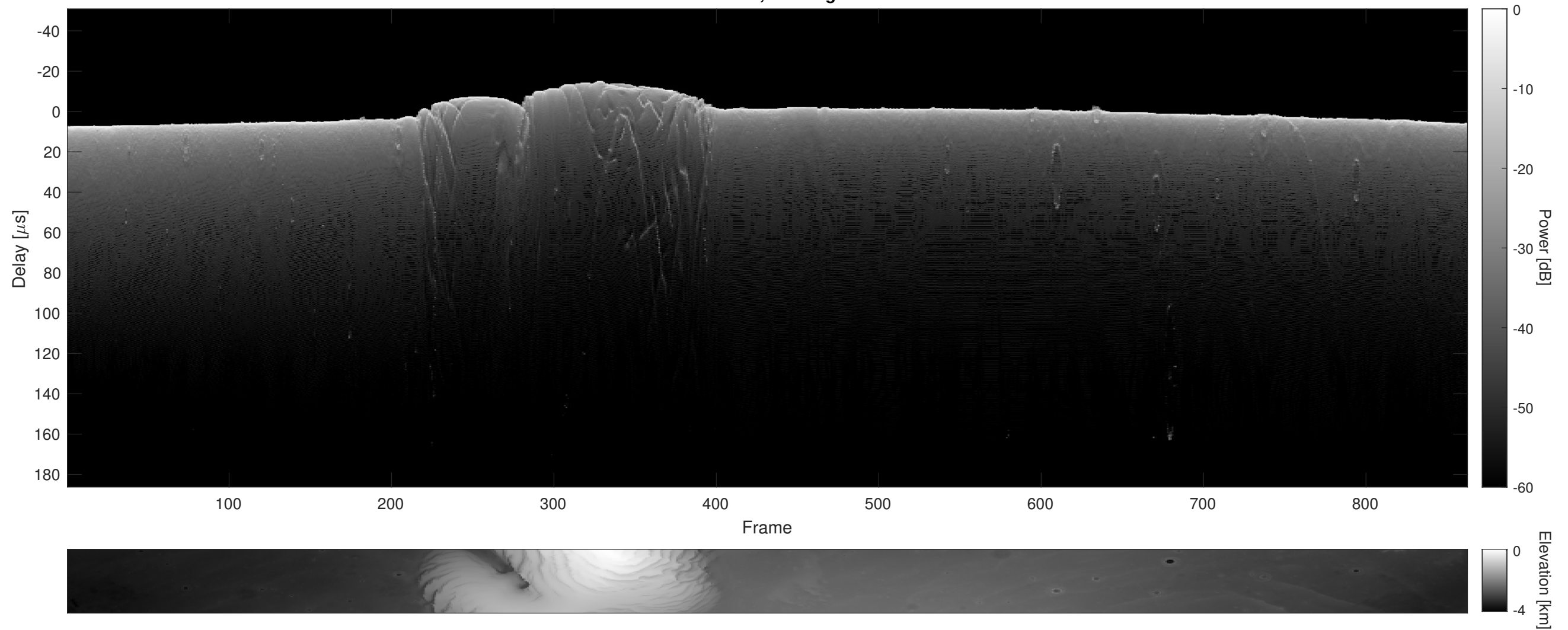
Orbit 15955, Cluttergram
