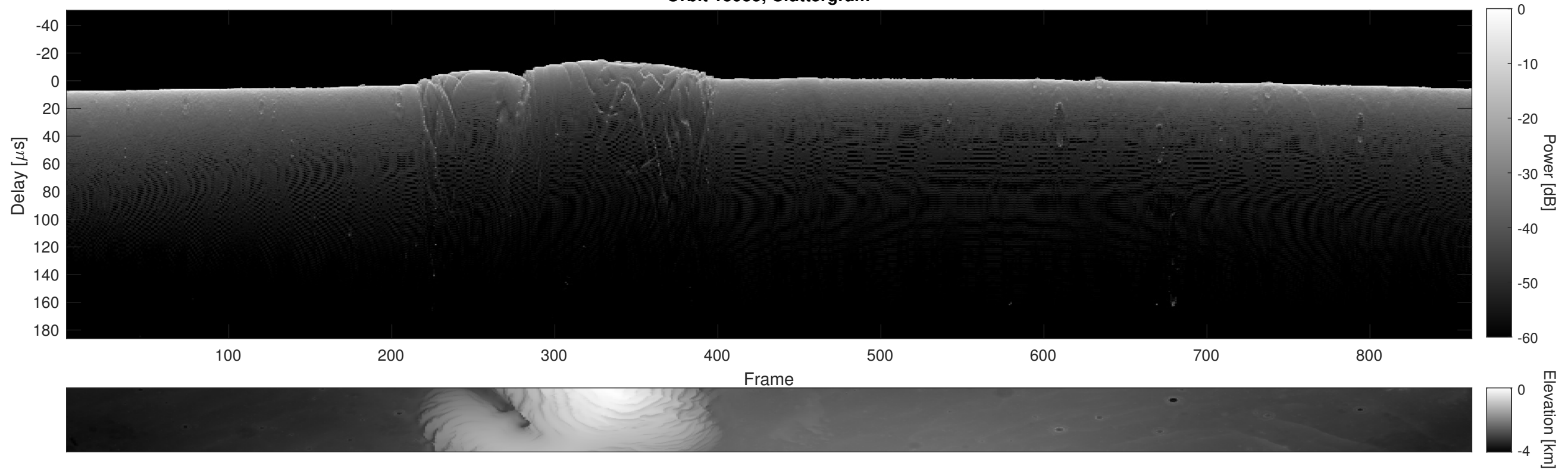
Orbit 15955, Cluttergram
