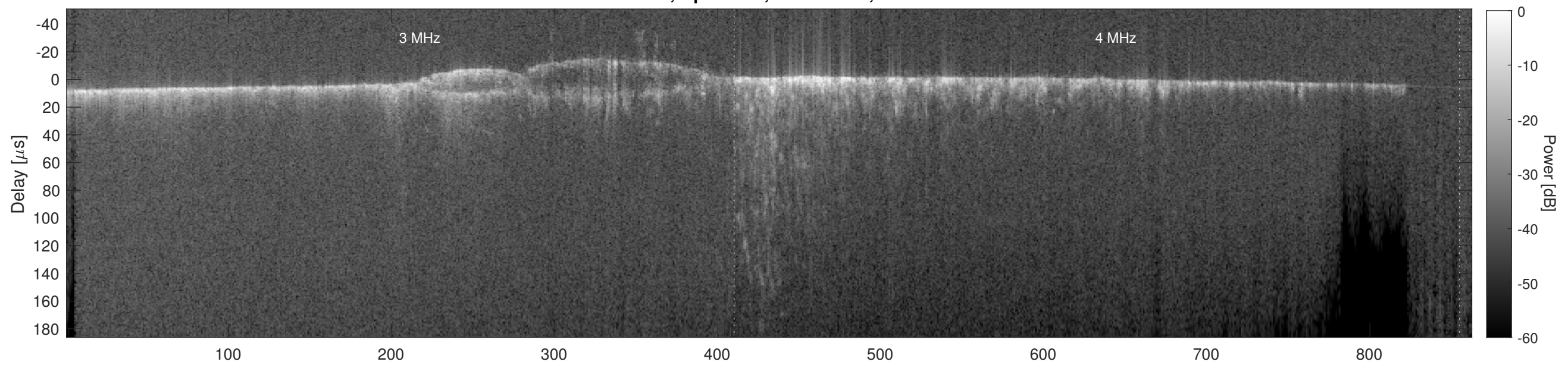
Orbit 15955, Cluttergram
