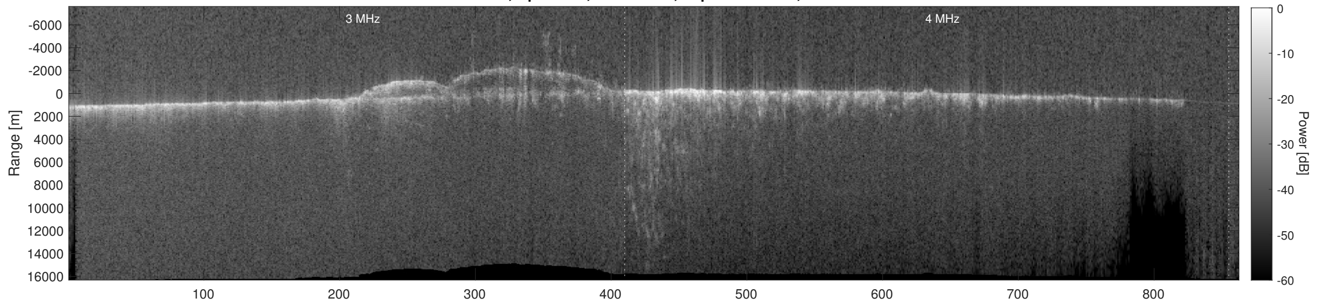
Orbit 15955, Depth-Corrected Cluttergram
