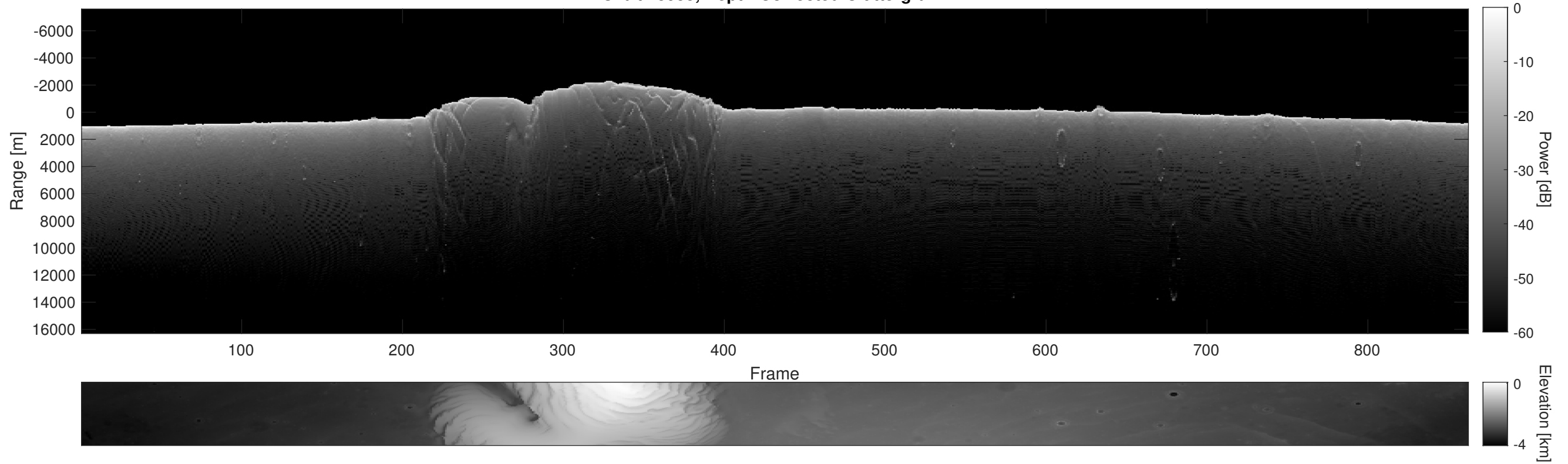
Orbit 15955, Depth-Corrected Cluttergram
