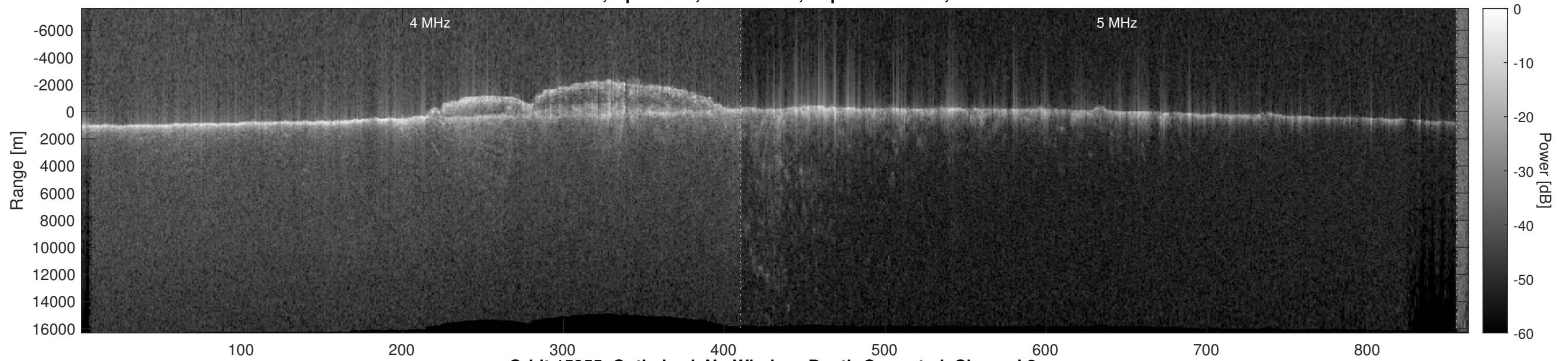
Orbit 15955, Optimized, No Window, Depth-Corrected, Channel 2
