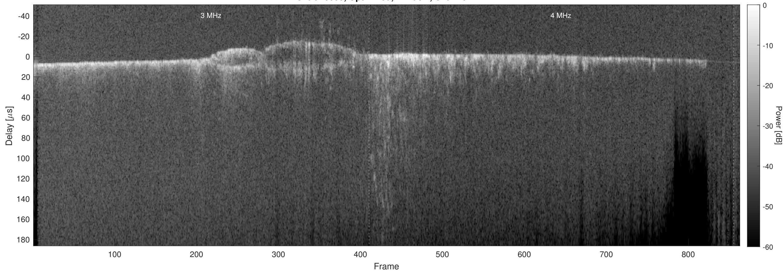
Orbit 15955, Optimized, Window, Channel 2
