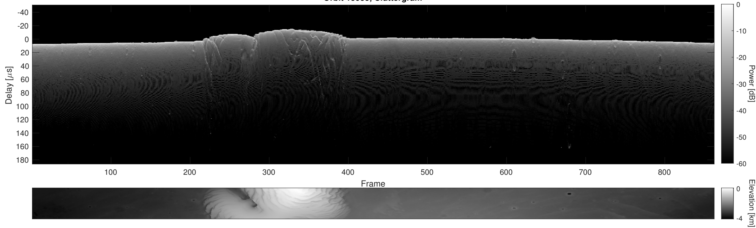
Orbit 15955, Cluttergram
