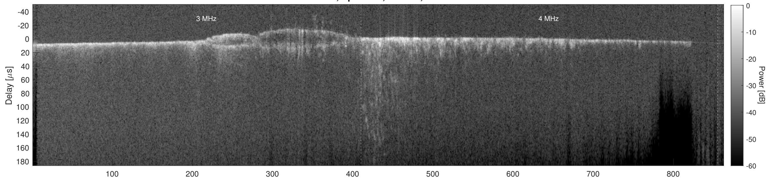
Orbit 15955, Cluttergram
