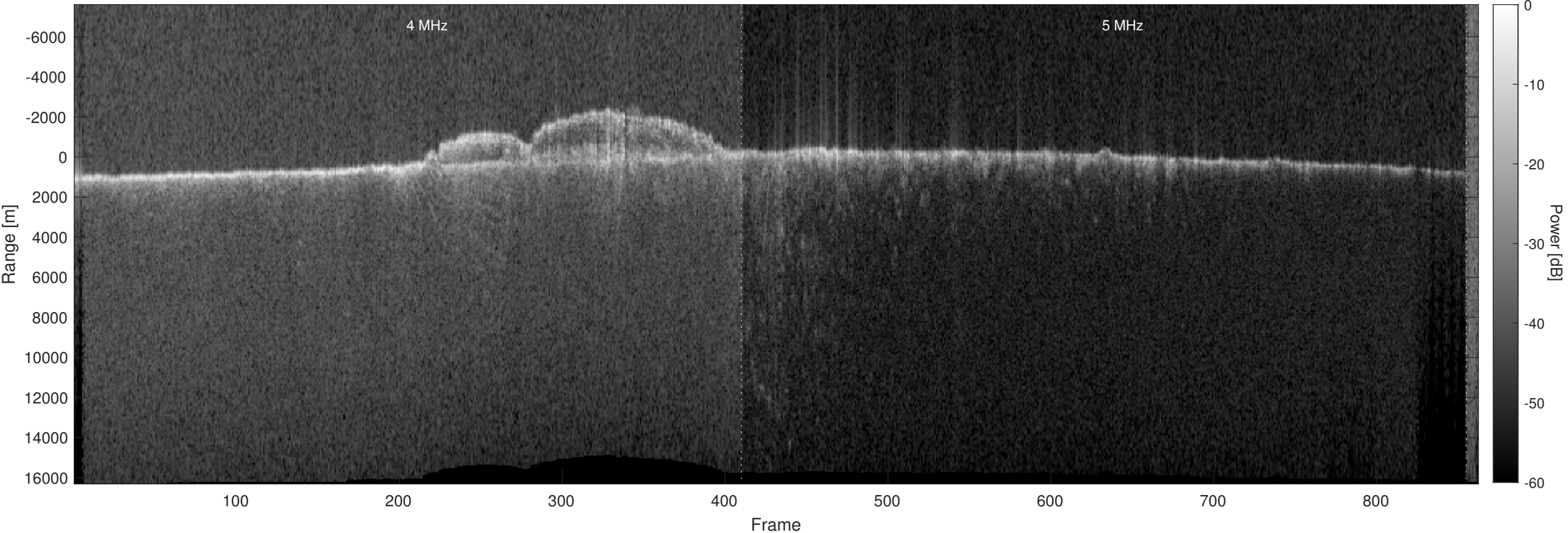
Orbit 15955, Optimized, Window, Depth-Corrected, Channel 2
