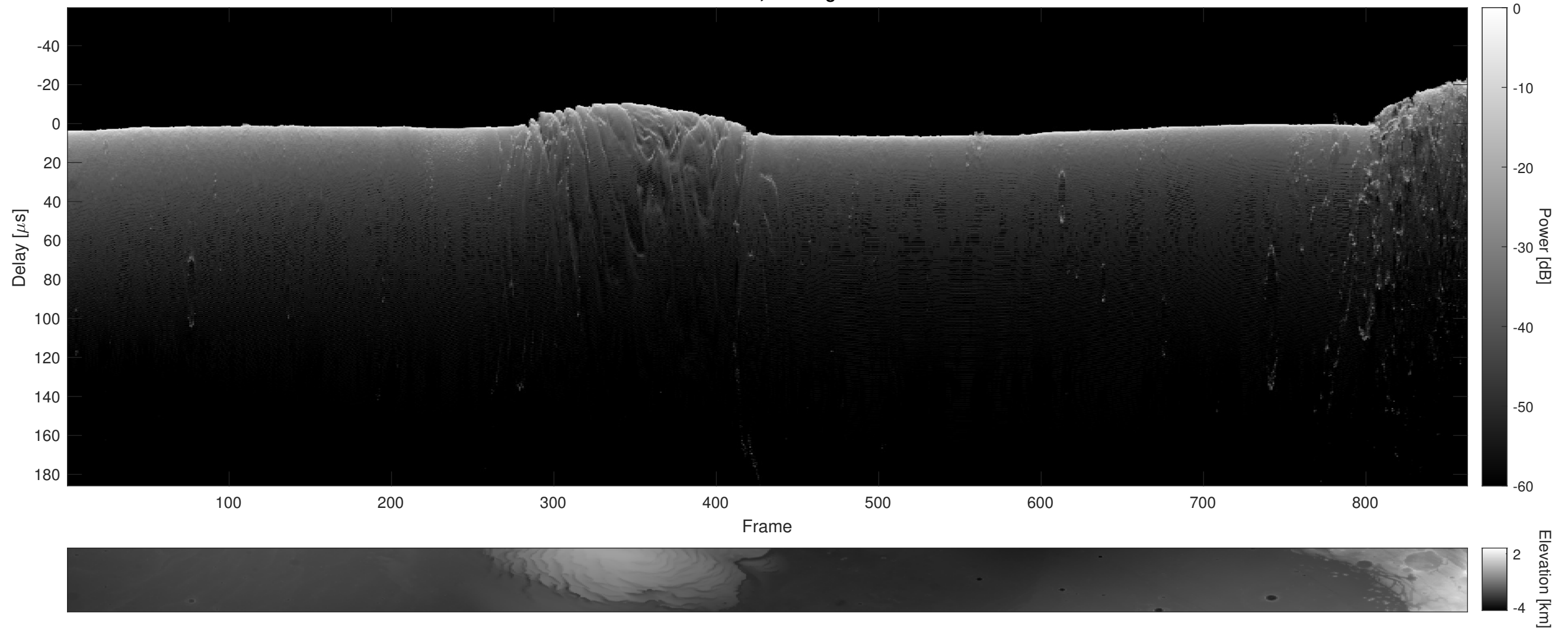
Orbit 15957, Cluttergram
