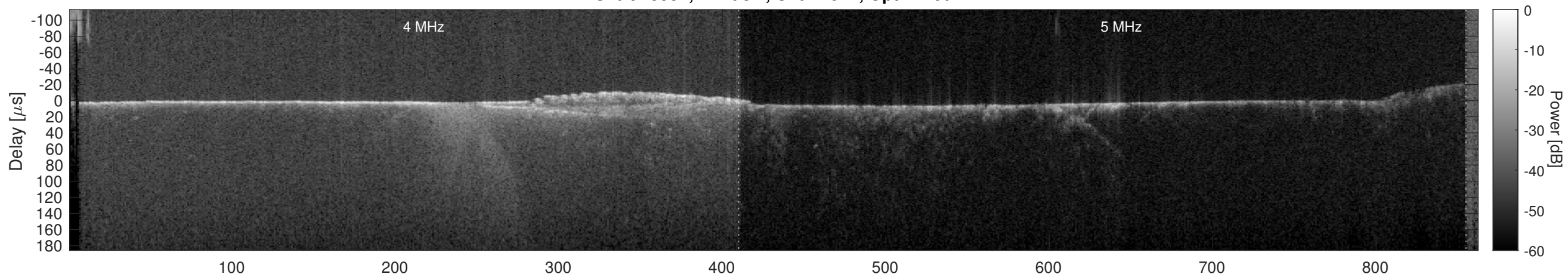
Orbit 15957, Cluttergram
