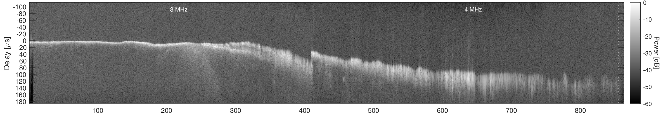
Orbit 15957, Window, Channel 2, Chapman
