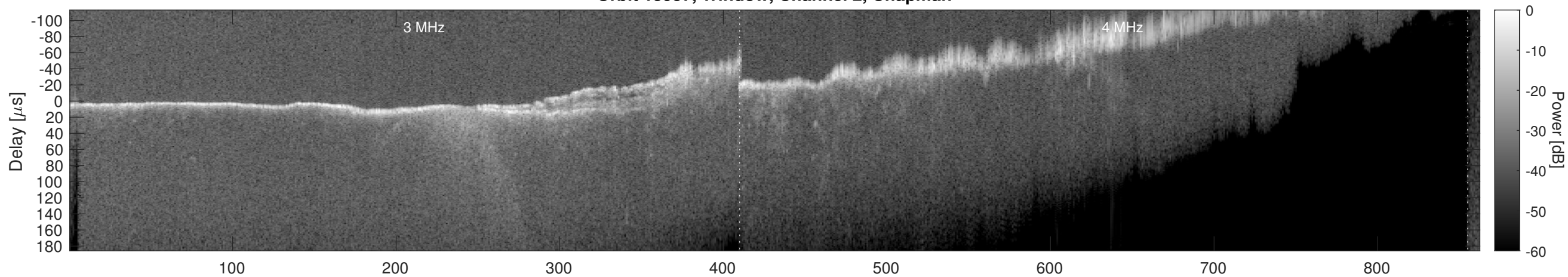
Orbit 15957, Window, Channel 2, Optimized
