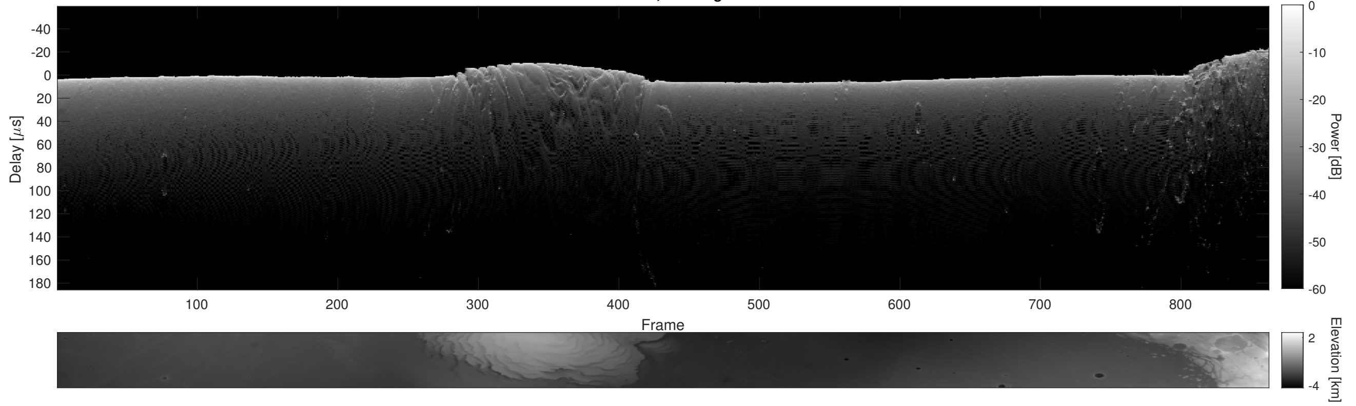
Orbit 15957, Cluttergram
