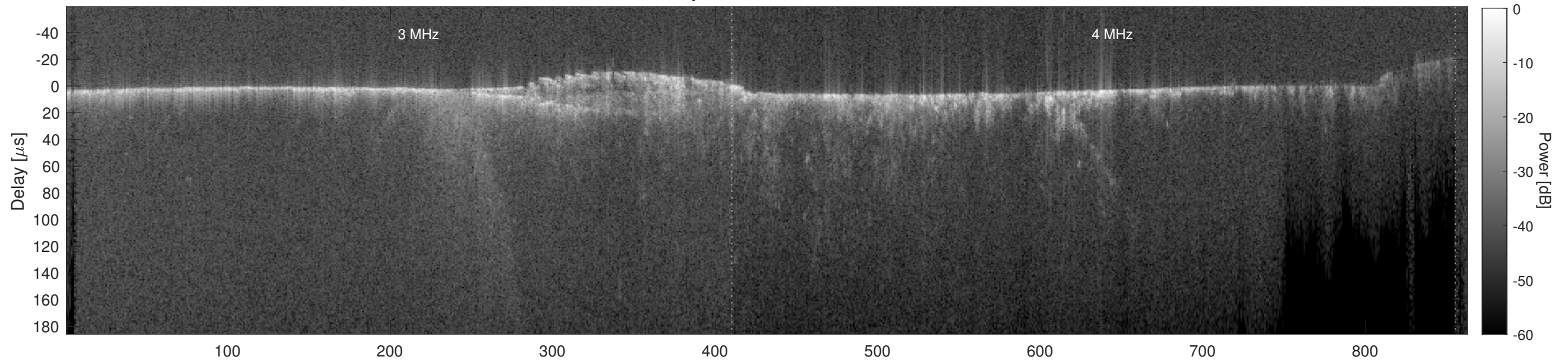
Orbit 15957, Cluttergram
